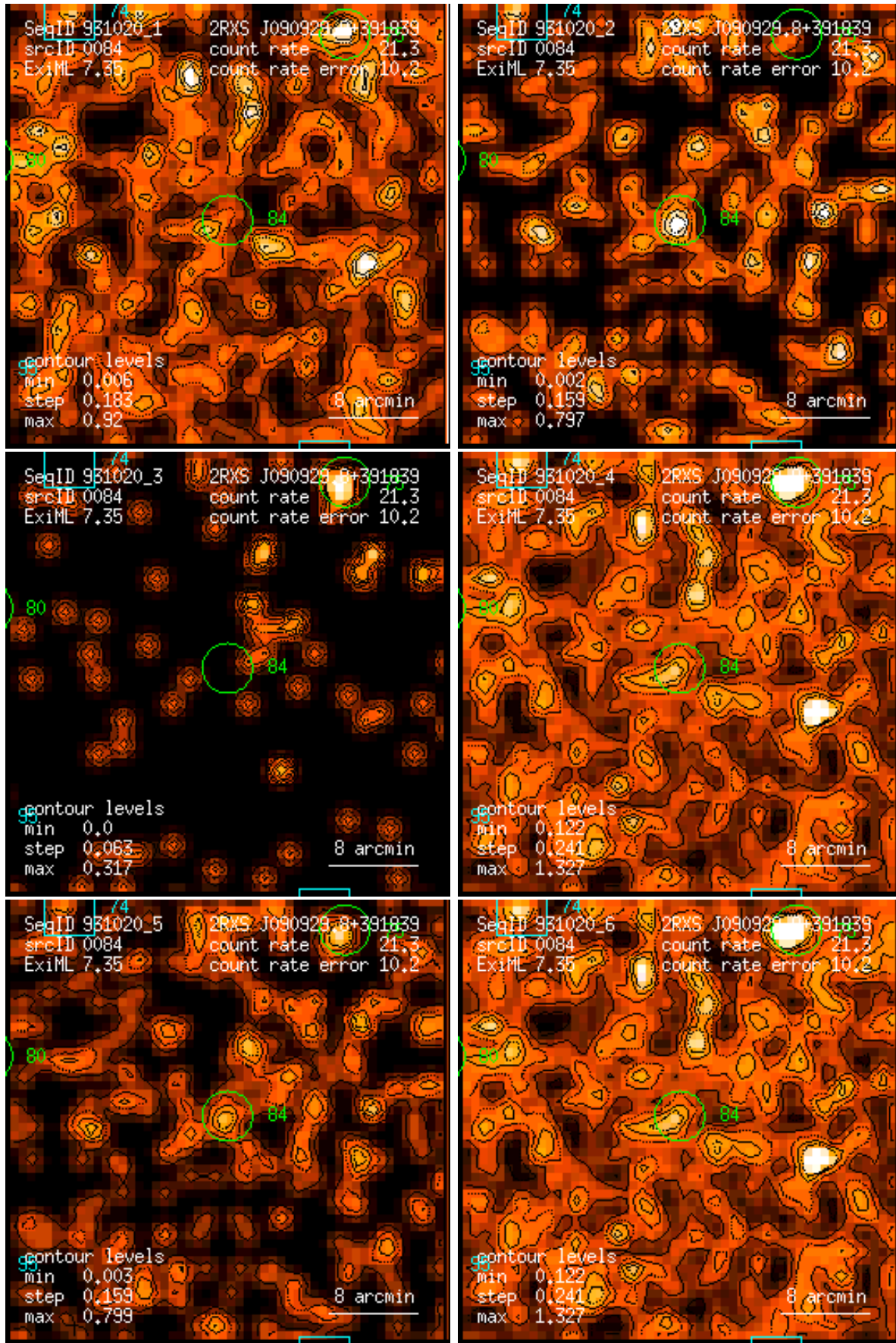
Figure 84: RASS 931020: detection 0084: band rate images, Gaussian filter: (1) PSPC channels 11 – 41, (2) 52 – 90, (3) 91 – 201, (4) 11 – 235, (5) 52 – 201, (6) 11 – 201. Broad band rates in counts/ks. Band rate contour levels in counts/ks/arcmin 2 .
