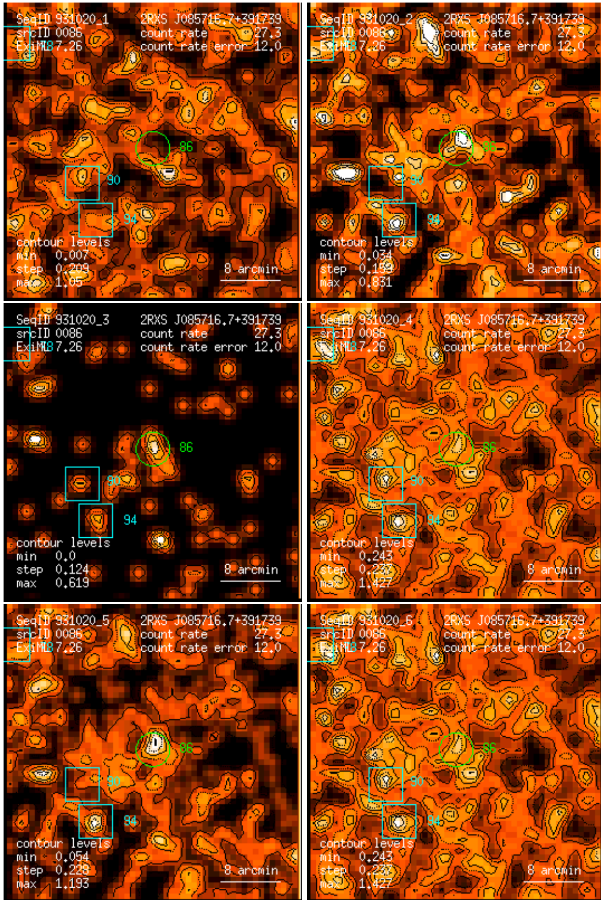
Figure 86: RASS 931020: detection 0086: band rate images, Gaussian filter: (1) PSPC channels 11 – 41, (2) 52 – 90, (3) 91 – 201, (4) 11 – 235, (5) 52 – 201, (6) 11 – 201. Broad band rates in counts/ks. Band rate contour levels in counts/ks/arcmin 2 .
