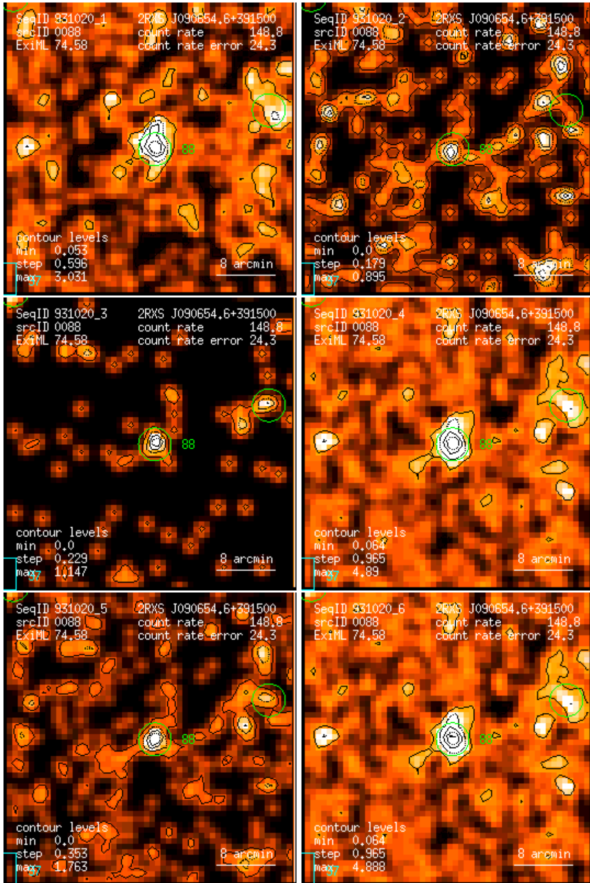
Figure 88: RASS 931020: detection 0088: band rate images, Gaussian filter: (1) PSPC channels 11 – 41, (2) 52 – 90, (3) 91 – 201, (4) 11 – 235, (5) 52 – 201, (6) 11 – 201. Broad band rates in counts/ks. Band rate contour levels in counts/ks/arcmin 2 .
