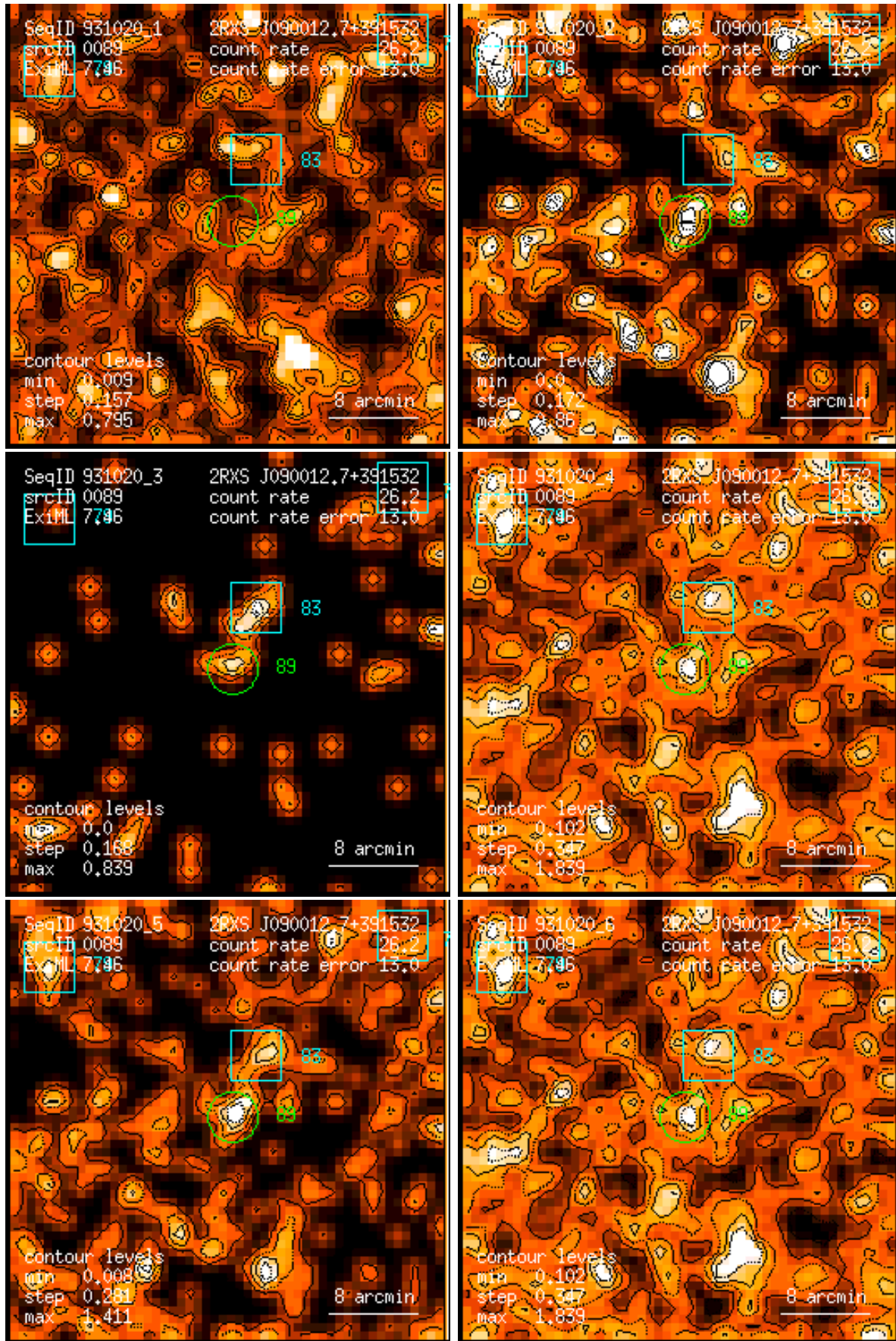
Figure 89: RASS 931020: detection 0089: band rate images, Gaussian filter: (1) PSPC channels 11 – 41, (2) 52 – 90, (3) 91 – 201, (4) 11 – 235, (5) 52 – 201, (6) 11 – 201. Broad band rates in counts/ks. Band rate contour levels in counts/ks/arcmin 2 .
