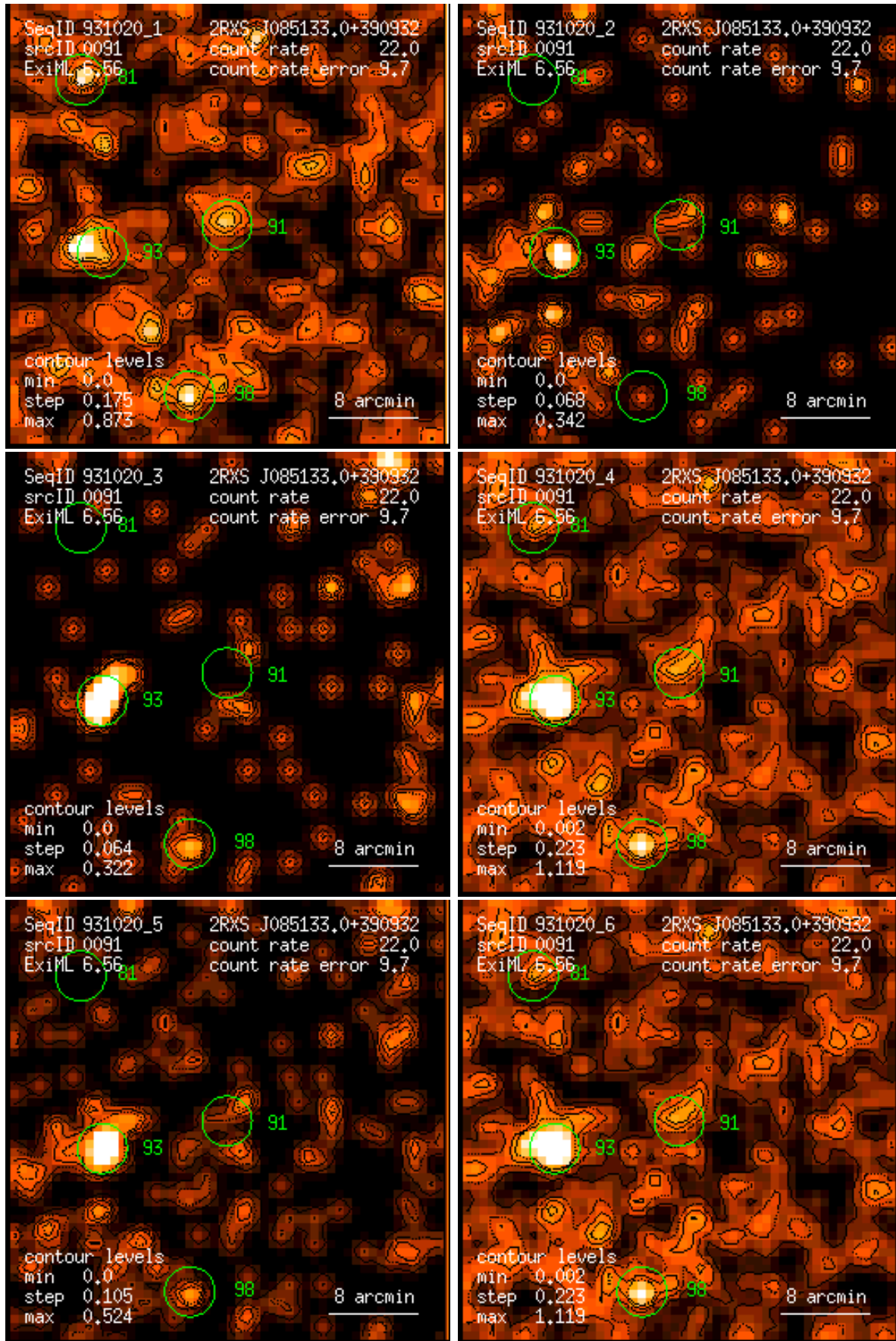
Figure 91: RASS 931020: detection 0091: band rate images, Gaussian filter: (1) PSPC channels 11 – 41, (2) 52 – 90, (3) 91 – 201, (4) 11 – 235, (5) 52 – 201, (6) 11 – 201. Broad band rates in counts/ks. Band rate contour levels in counts/ks/arcmin 2 .
