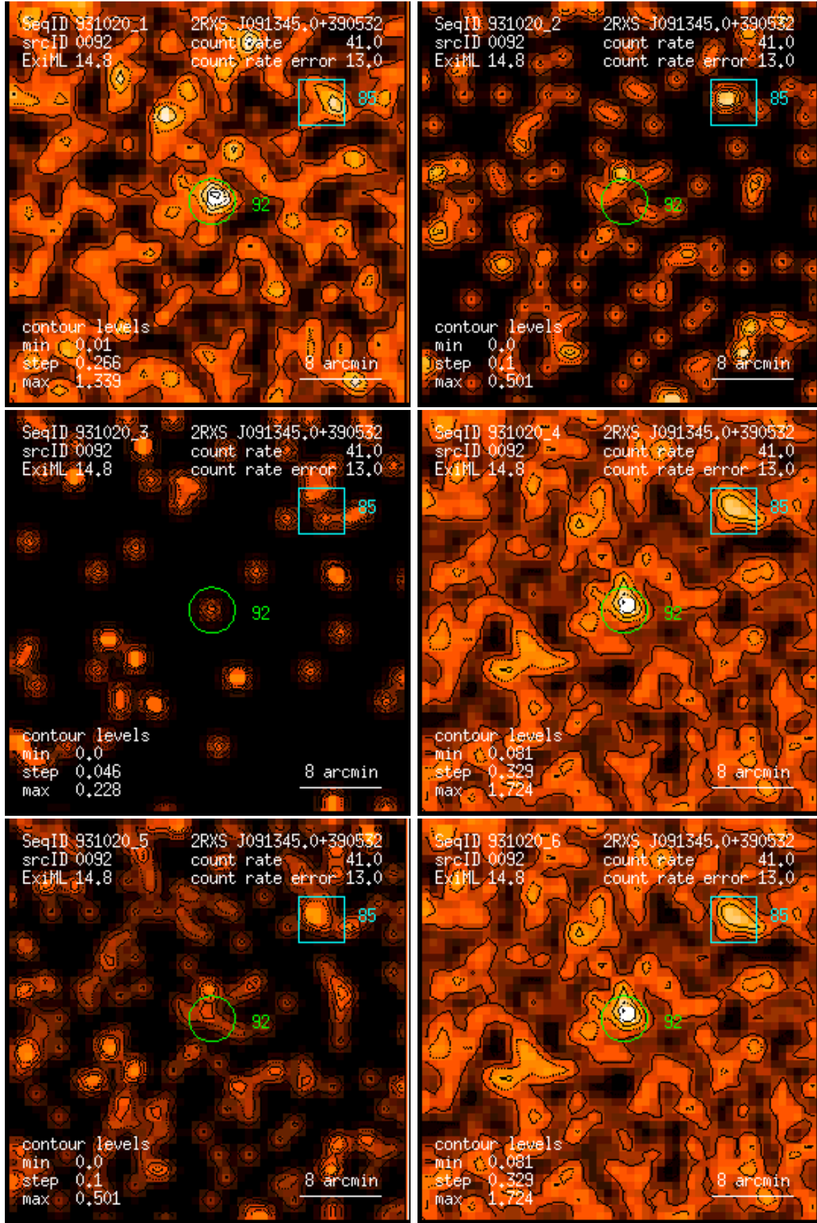
Figure 92: RASS 931020: detection 0092: band rate images, Gaussian filter: (1) PSPC channels 11 – 41, (2) 52 – 90, (3) 91 – 201, (4) 11 – 235, (5) 52 – 201, (6) 11 – 201. Broad band rates in counts/ks. Band rate contour levels in counts/ks/arcmin 2 .
