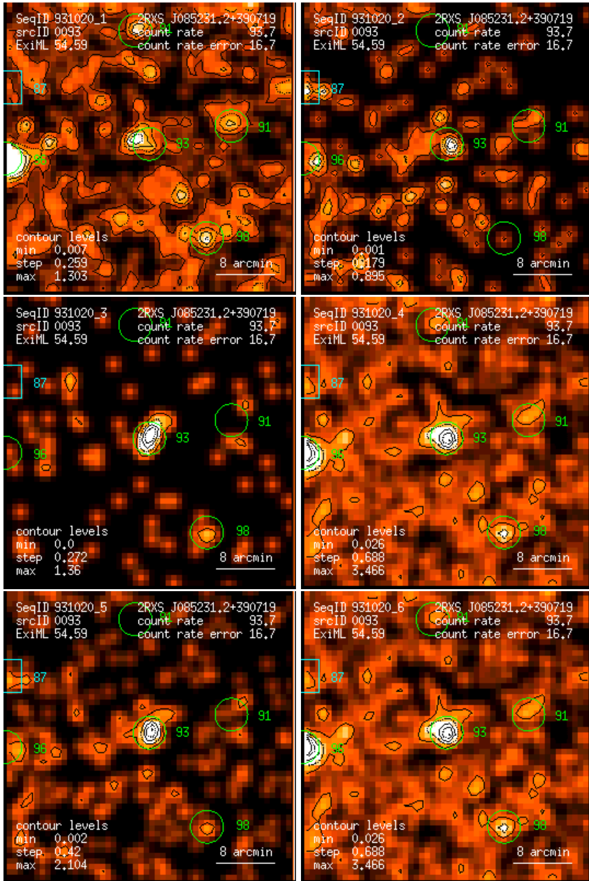
Figure 93: RASS 931020: detection 0093: band rate images, Gaussian filter: (1) PSPC channels 11 – 41, (2) 52 – 90, (3) 91 – 201, (4) 11 – 235, (5) 52 – 201, (6) 11 – 201. Broad band rates in counts/ks. Band rate contour levels in counts/ks/arcmin 2 .
