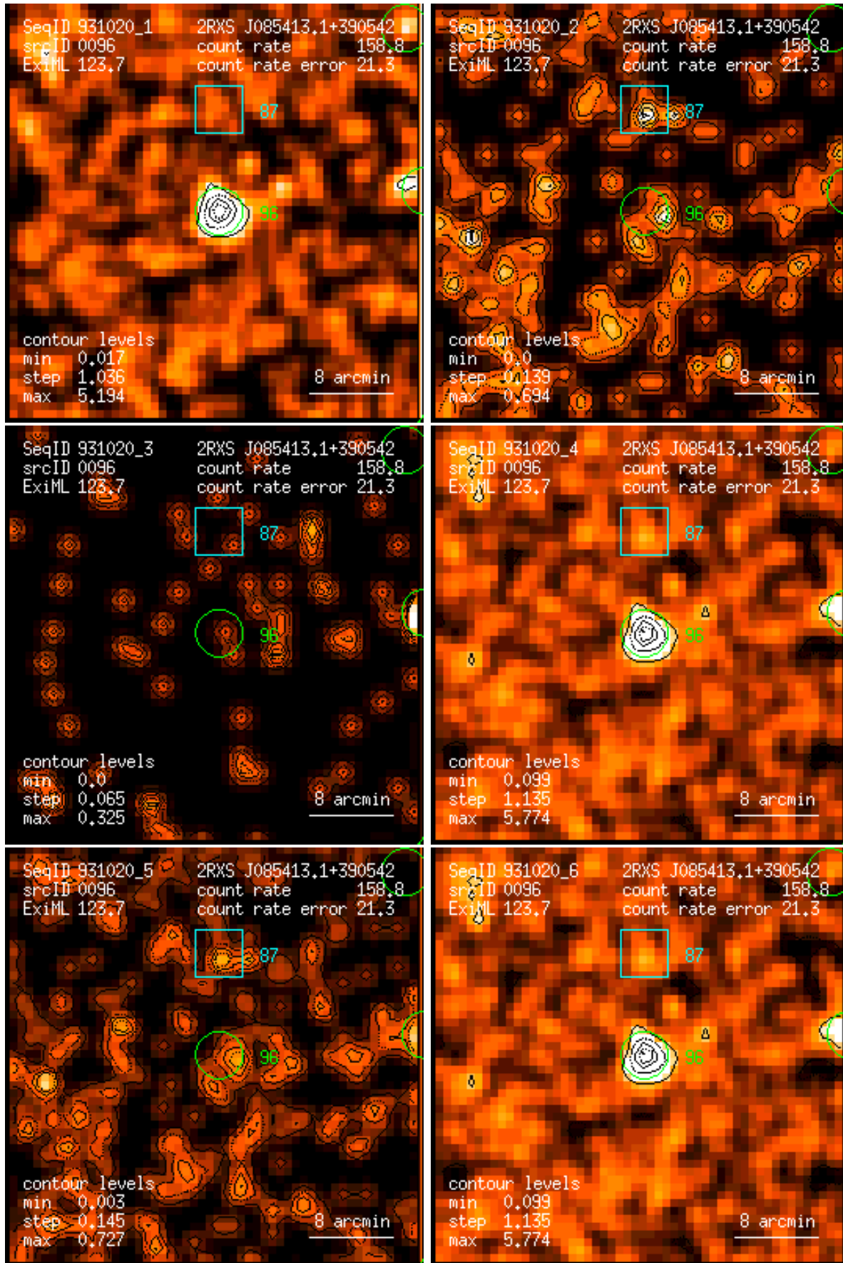
Figure 96: RASS 931020: detection 0096: band rate images, Gaussian filter: (1) PSPC channels 11 – 41, (2) 52 – 90, (3) 91 – 201, (4) 11 – 235, (5) 52 – 201, (6) 11 – 201. Broad band rates in counts/ks. Band rate contour levels in counts/ks/arcmin 2 .
