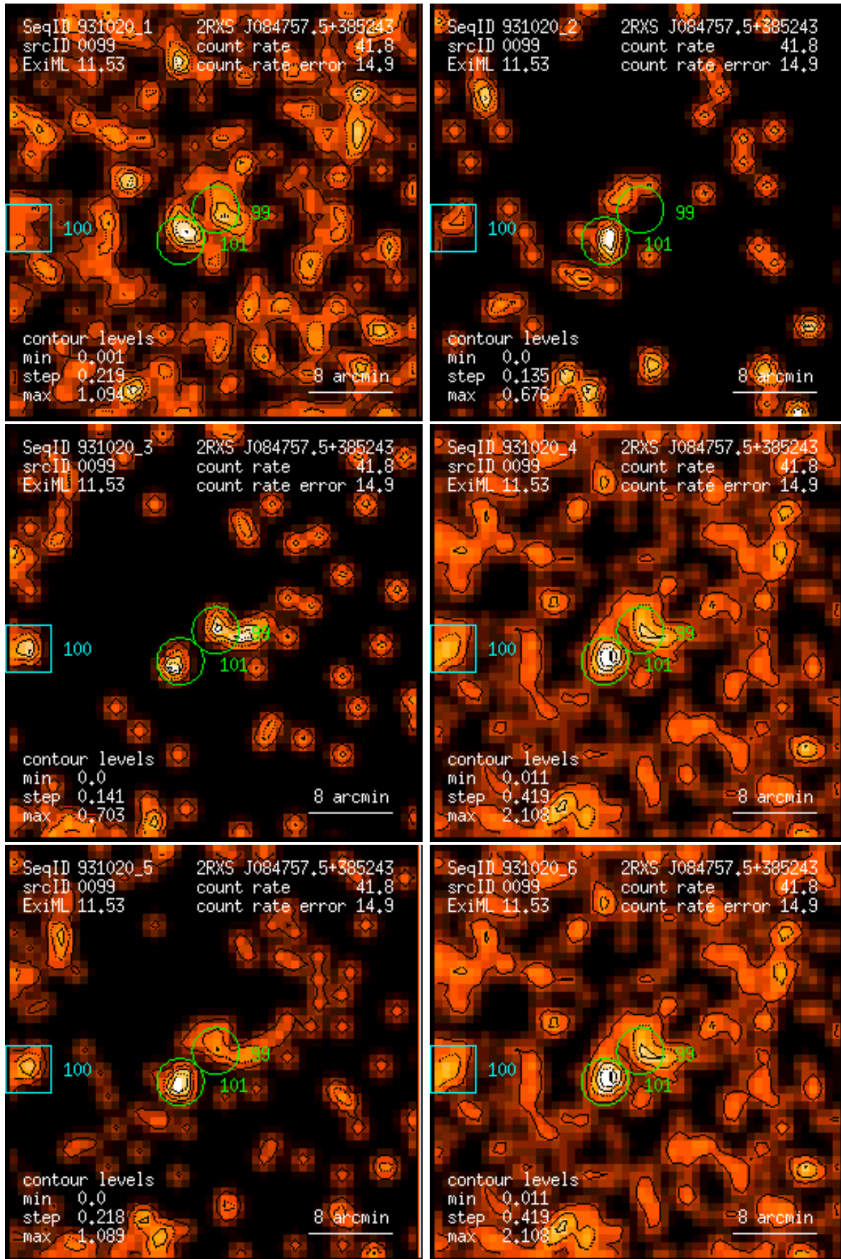
Figure 99: RASS 931020: detection 0099: band rate images, Gaussian filter: (1) PSPC channels 11 – 41, (2) 52 – 90, (3) 91 – 201, (4) 11 – 235, (5) 52 – 201, (6) 11 – 201. Broad band rates in counts/ks. Band rate contour levels in counts/ks/arcmin 2 .
