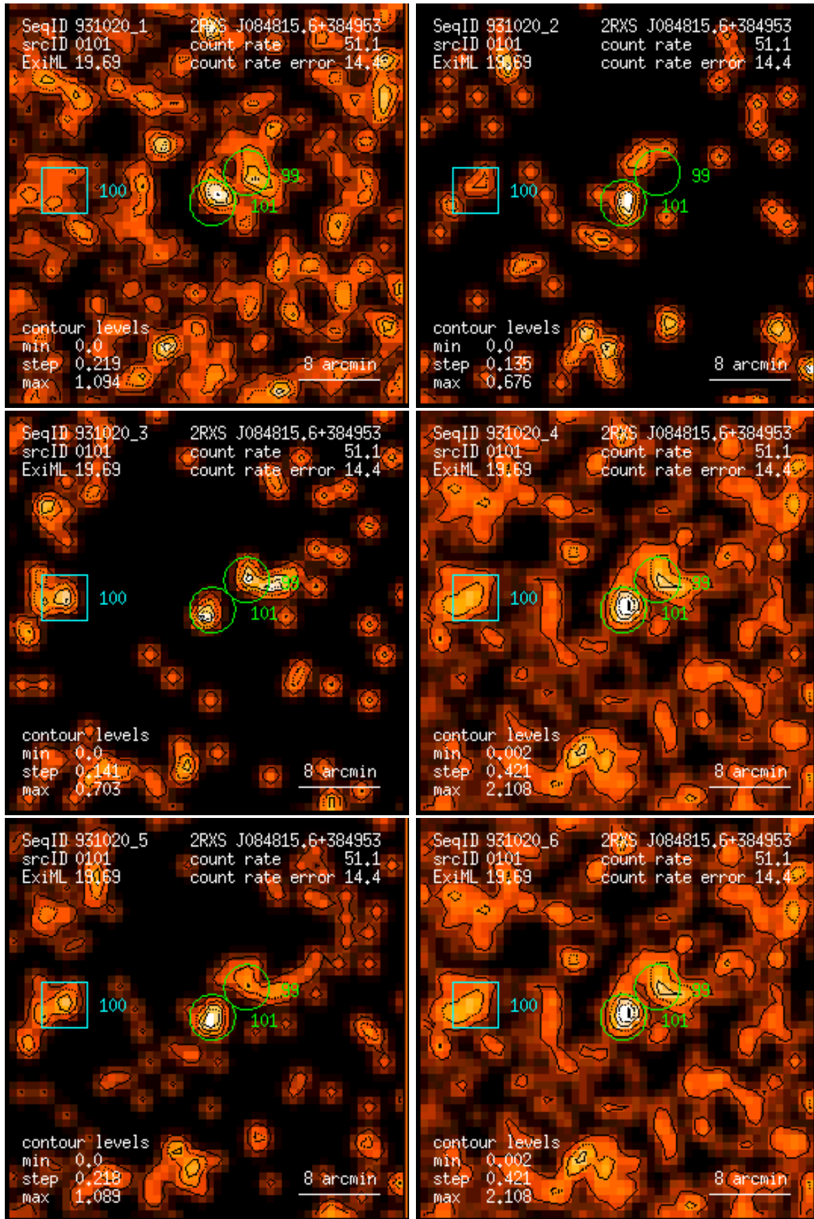
Figure 101: RASS 931020: detection 0101: band rate images, Gaussian filter: (1) PSPC channels 11 – 41, (2) 52 – 90, (3) 91 – 201, (4) 11 – 235, (5) 52 – 201, (6) 11 – 201. Broad band rates in counts/ks. Band rate contour levels in counts/ks/arcmin 2 .
