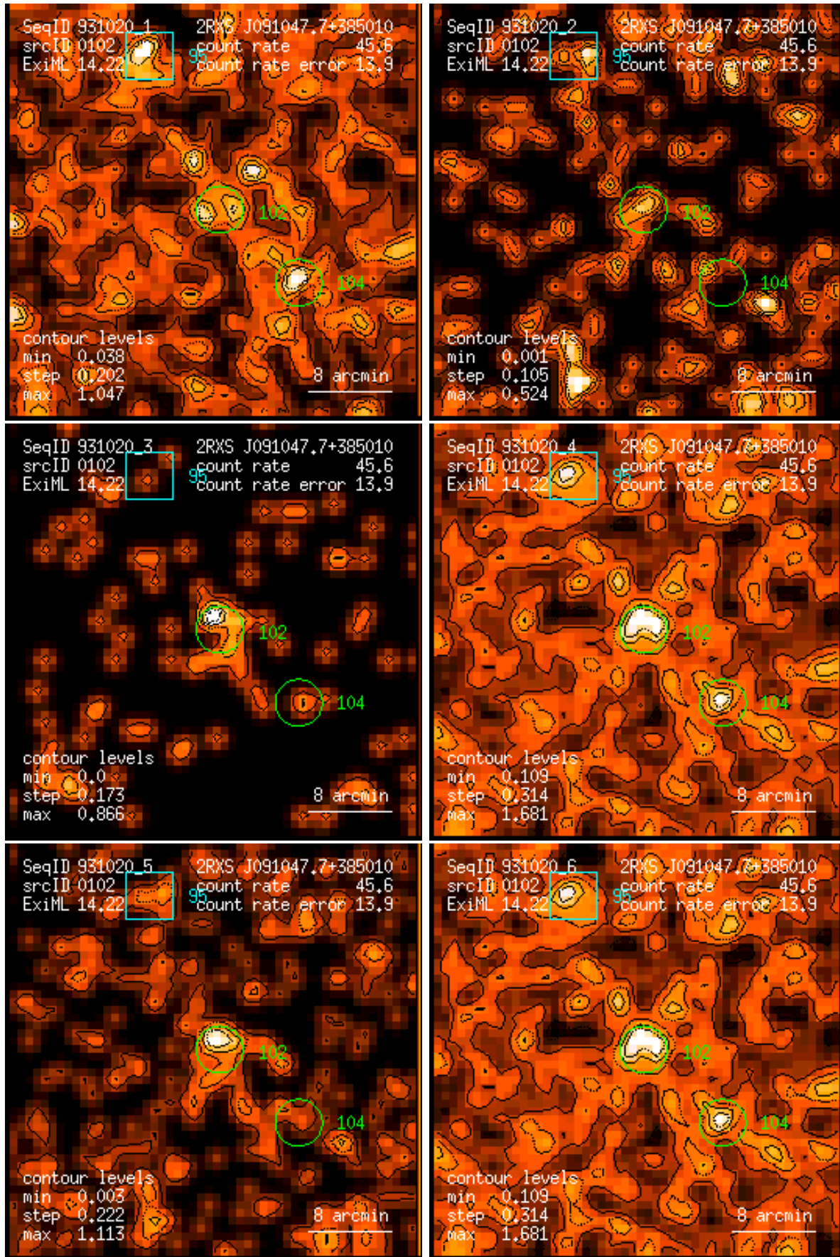
Figure 102: RASS 931020: detection 0102: band rate images, Gaussian filter: (1) PSPC channels 11 – 41, (2) 52 – 90, (3) 91 – 201, (4) 11 – 235, (5) 52 – 201, (6) 11 – 201. Broad band rates in counts/ks. Band rate contour levels in counts/ks/arcmin 2 .
