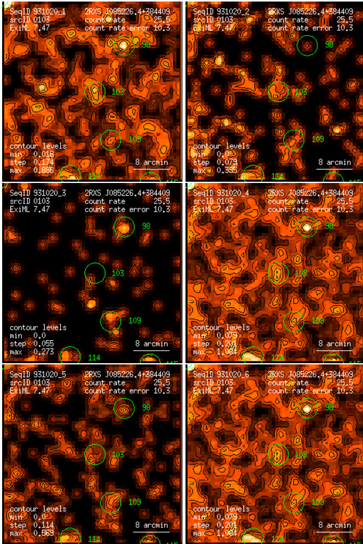
Figure 103: RASS 931020: detection 0103: band rate images, Gaussian filter: (1) PSPC channels 11 – 41, (2) 52 – 90, (3) 91 – 201, (4) 11 – 235, (5) 52 – 201, (6) 11 – 201. Broad band rates in counts/ks. Band rate contour levels in counts/ks/arcmin 2 .
