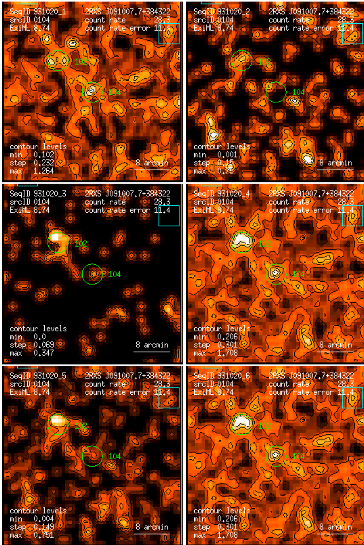
Figure 104: RASS 931020: detection 0104: band rate images, Gaussian filter: (1) PSPC channels 11 – 41, (2) 52 – 90, (3) 91 – 201, (4) 11 – 235, (5) 52 – 201, (6) 11 – 201. Broad band rates in counts/ks. Band rate contour levels in counts/ks/arcmin 2 .
