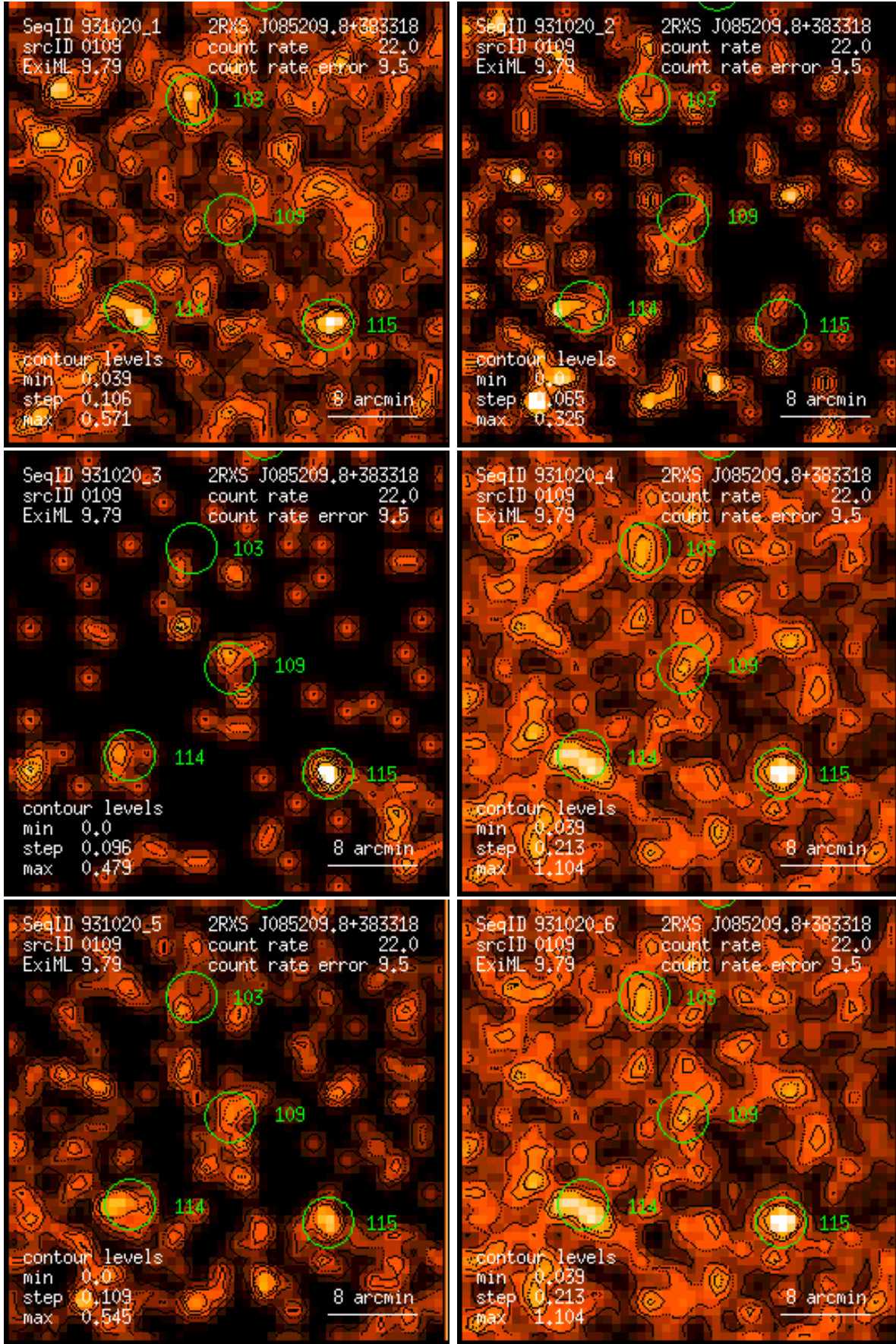
Figure 109: RASS 931020: detection 0109: band rate images, Gaussian filter: (1) PSPC channels 11 – 41, (2) 52 – 90, (3) 91 – 201, (4) 11 – 235, (5) 52 – 201, (6) 11 – 201. Broad band rates in counts/ks. Band rate contour levels in counts/ks/arcmin 2 .
