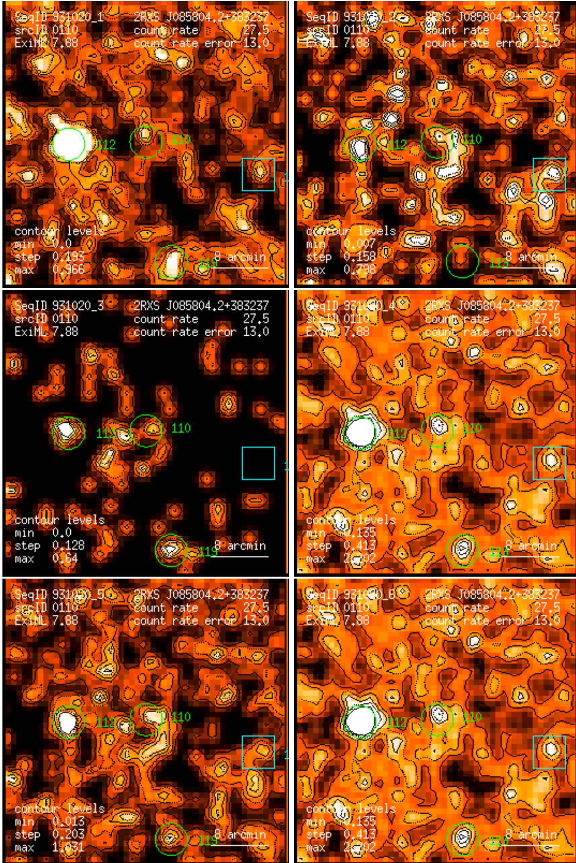
Figure 110: RASS 931020: detection 0110: band rate images, Gaussian filter: (1) PSPC channels 11 – 41, (2) 52 – 90, (3) 91 – 201, (4) 11 – 235, (5) 52 – 201, (6) 11 – 201. Broad band rates in counts/ks. Band rate contour levels in counts/ks/arcmin 2 .
