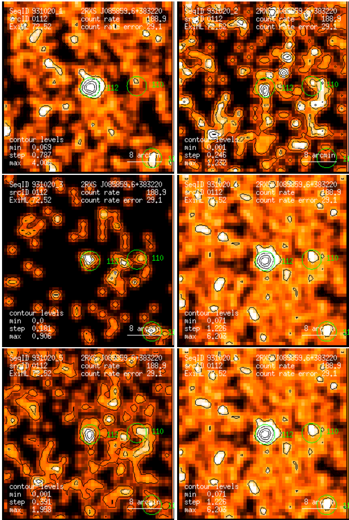
Figure 112: RASS 931020: detection 0112: band rate images, Gaussian filter: (1) PSPC channels 11 – 41, (2) 52 – 90, (3) 91 – 201, (4) 11 – 235, (5) 52 – 201, (6) 11 – 201. Broad band rates in counts/ks. Band rate contour levels in counts/ks/arcmin 2 .
