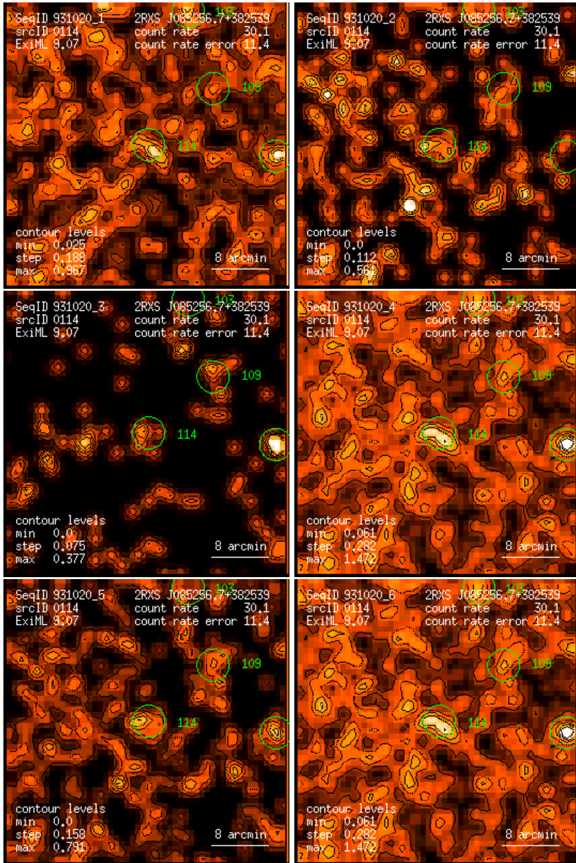
Figure 114: RASS 931020: detection 0114: band rate images, Gaussian filter: (1) PSPC channels 11 – 41, (2) 52 – 90, (3) 91 – 201, (4) 11 – 235, (5) 52 – 201, (6) 11 – 201. Broad band rates in counts/ks. Band rate contour levels in counts/ks/arcmin 2 .
