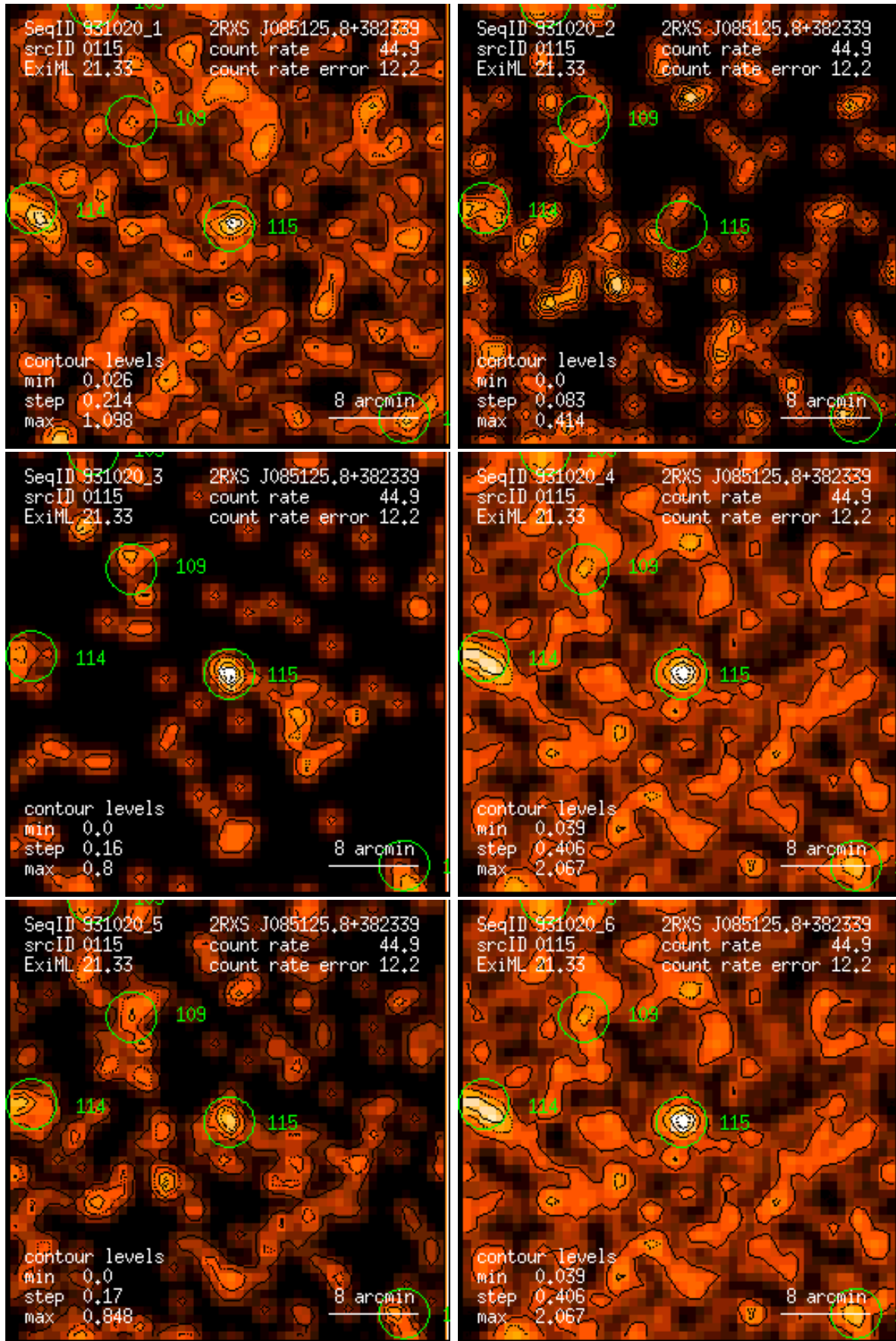
Figure 115: RASS 931020: detection 0115: band rate images, Gaussian filter: (1) PSPC channels 11 – 41, (2) 52 – 90, (3) 91 – 201, (4) 11 – 235, (5) 52 – 201, (6) 11 – 201. Broad band rates in counts/ks. Band rate contour levels in counts/ks/arcmin 2 .
