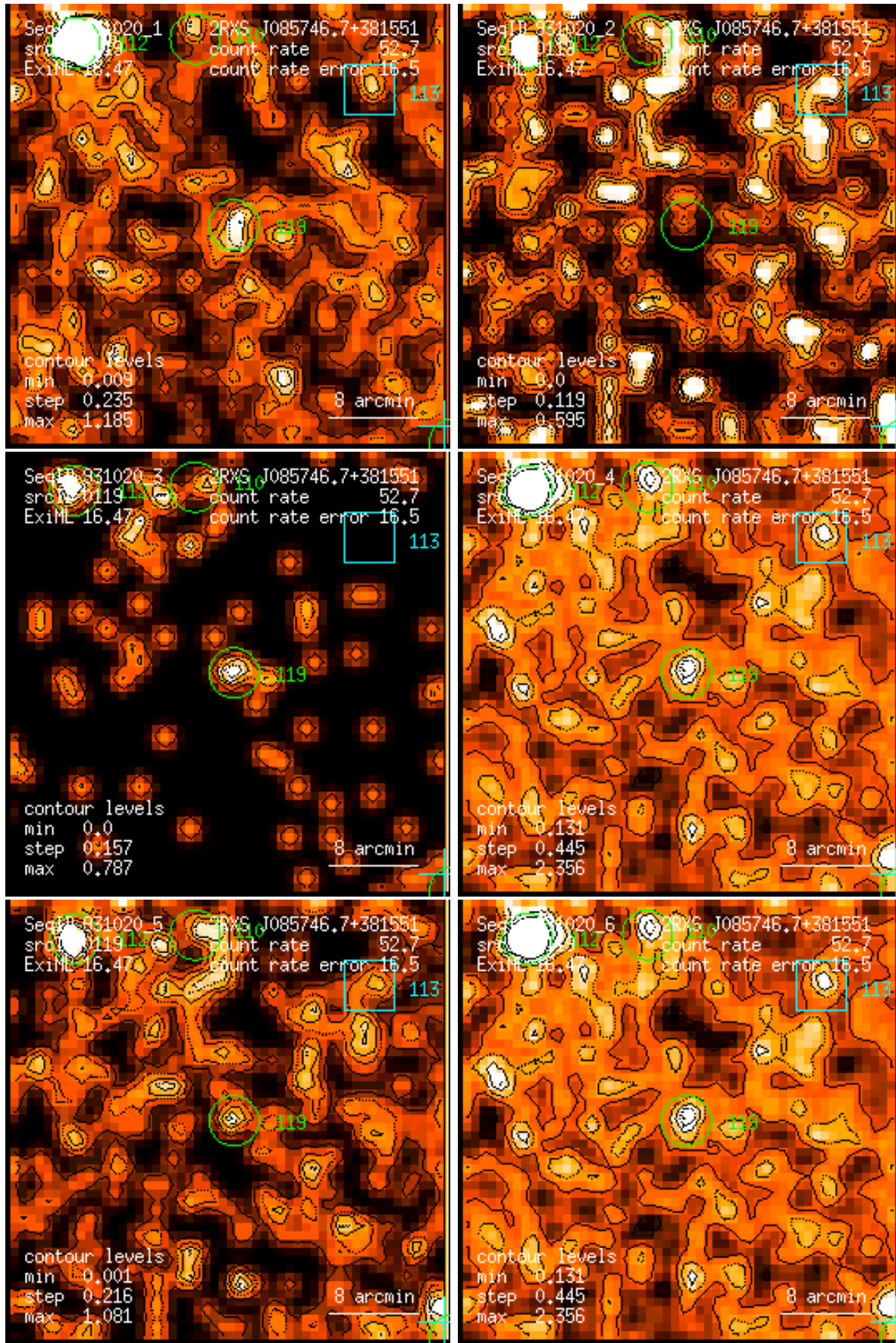
Figure 119: RASS 931020: detection 0119: band rate images, Gaussian filter: (1) PSPC channels 11 – 41, (2) 52 – 90, (3) 91 – 201, (4) 11 – 235, (5) 52 – 201, (6) 11 – 201. Broad band rates in counts/ks. Band rate contour levels in counts/ks/arcmin 2 .
