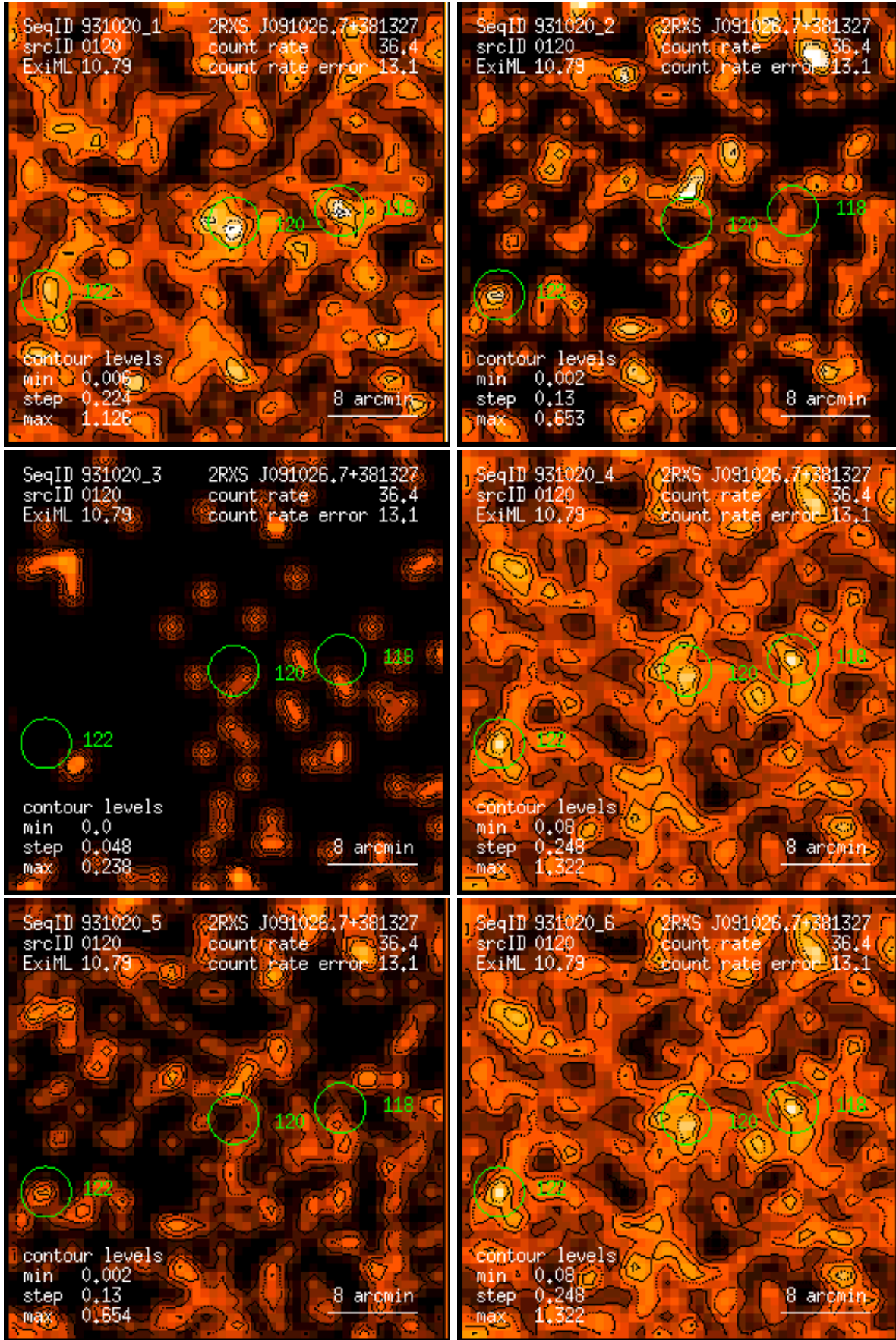
Figure 120: RASS 931020: detection 0120: band rate images, Gaussian filter: (1) PSPC channels 11 – 41, (2) 52 – 90, (3) 91 – 201, (4) 11 – 235, (5) 52 – 201, (6) 11 – 201. Broad band rates in counts/ks. Band rate contour levels in counts/ks/arcmin 2 .
