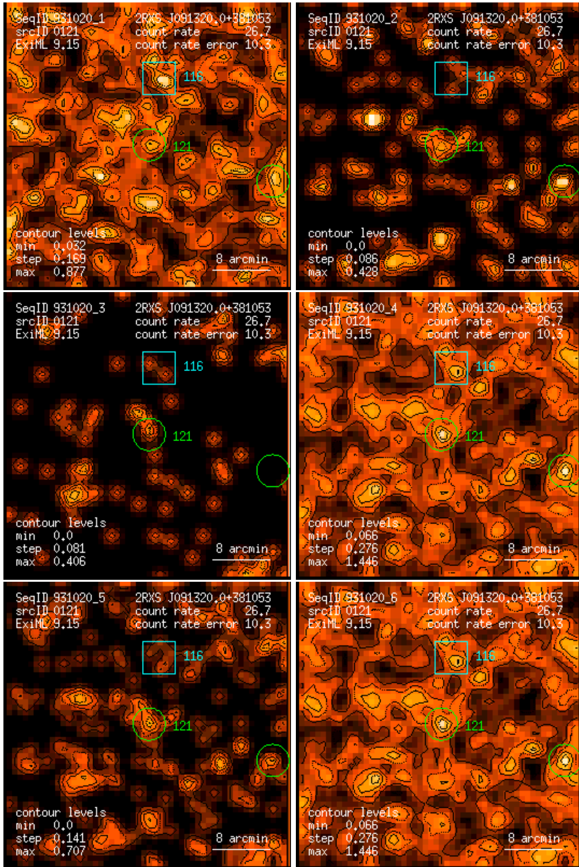
Figure 121: RASS 931020: detection 0121: band rate images, Gaussian filter: (1) PSPC channels 11 – 41, (2) 52 – 90, (3) 91 – 201, (4) 11 – 235, (5) 52 – 201, (6) 11 – 201. Broad band rates in counts/ks. Band rate contour levels in counts/ks/arcmin 2 .
