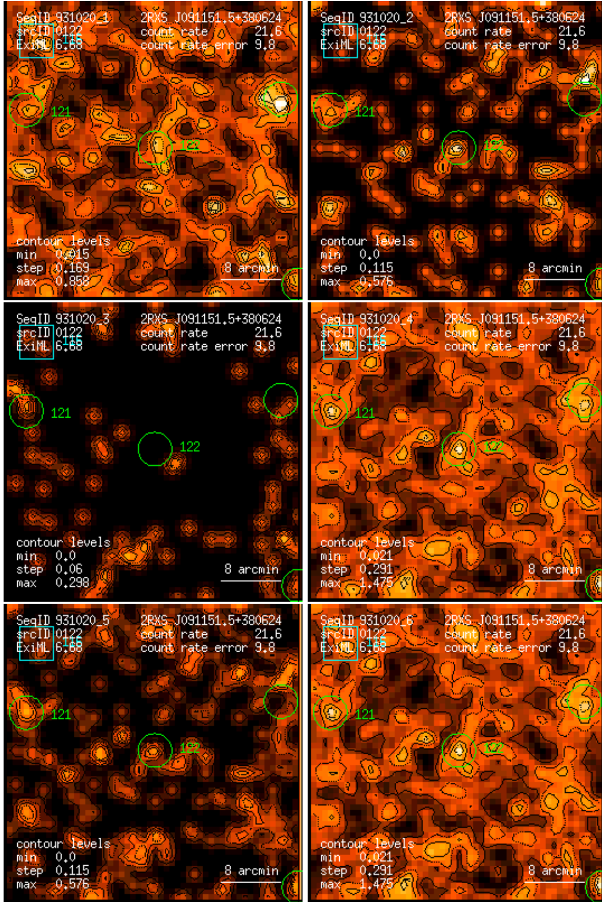
Figure 122: RASS 931020: detection 0122: band rate images, Gaussian filter: (1) PSPC channels 11 – 41, (2) 52 – 90, (3) 91 – 201, (4) 11 – 235, (5) 52 – 201, (6) 11 – 201. Broad band rates in counts/ks. Band rate contour levels in counts/ks/arcmin 2 .
