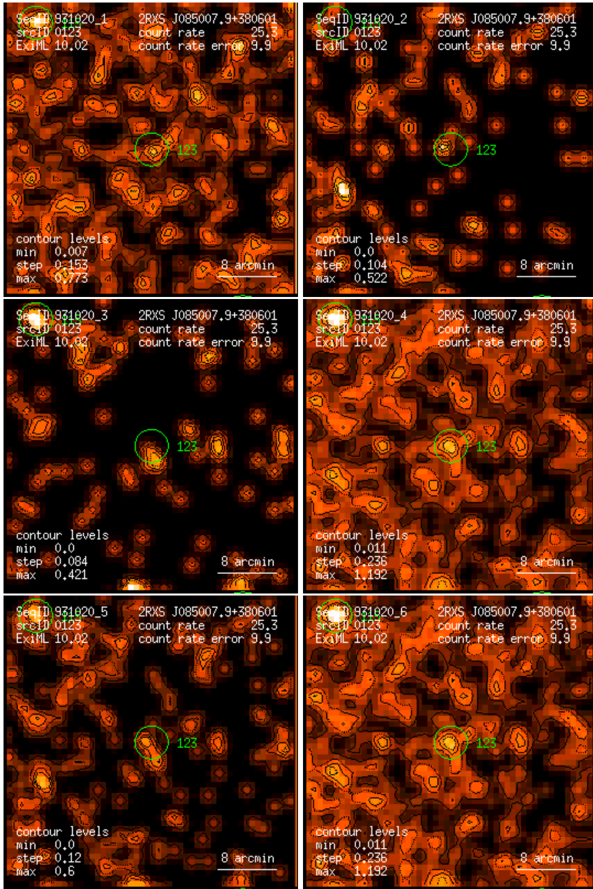
Figure 123: RASS 931020: detection 0123: band rate images, Gaussian filter: (1) PSPC channels 11 – 41, (2) 52 – 90, (3) 91 – 201, (4) 11 – 235, (5) 52 – 201, (6) 11 – 201. Broad band rates in counts/ks. Band rate contour levels in counts/ks/arcmin 2 .
