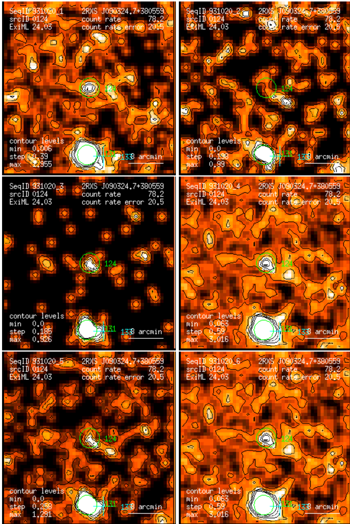
Figure 124: RASS 931020: detection 0124: band rate images, Gaussian filter: (1) PSPC channels 11 – 41, (2) 52 – 90, (3) 91 – 201, (4) 11 – 235, (5) 52 – 201, (6) 11 – 201. Broad band rates in counts/ks. Band rate contour levels in counts/ks/arcmin 2 .
