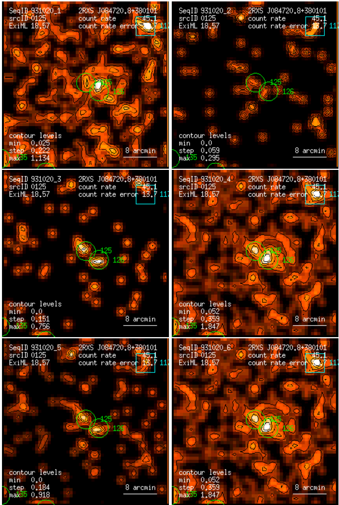
Figure 125: RASS 931020: detection 0125: band rate images, Gaussian filter: (1) PSPC channels 11 – 41, (2) 52 – 90, (3) 91 – 201, (4) 11 – 235, (5) 52 – 201, (6) 11 – 201. Broad band rates in counts/ks. Band rate contour levels in counts/ks/arcmin 2 .
