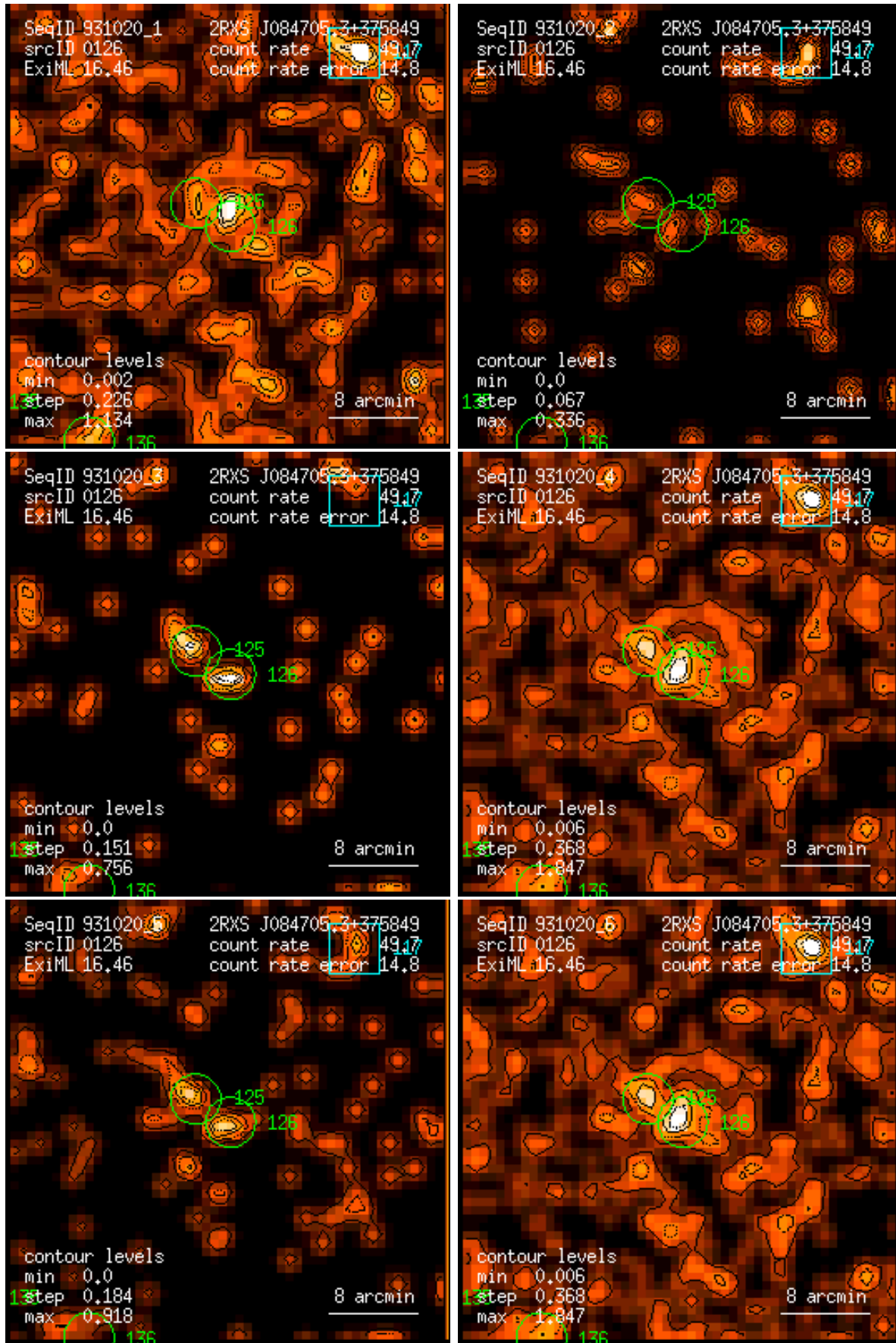
Figure 126: RASS 931020: detection 0126: band rate images, Gaussian filter: (1) PSPC channels 11 – 41, (2) 52 – 90, (3) 91 – 201, (4) 11 – 235, (5) 52 – 201, (6) 11 – 201. Broad band rates in counts/ks. Band rate contour levels in counts/ks/arcmin 2 .
