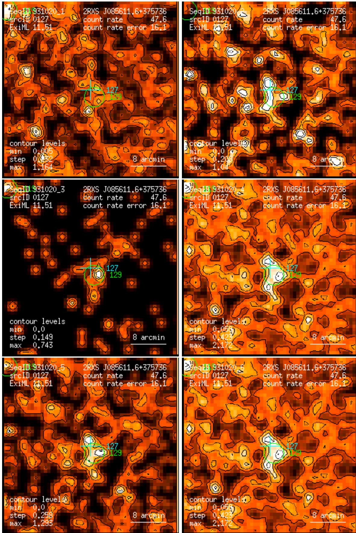
Figure 127: RASS 931020: detection 0127: band rate images, Gaussian filter: (1) PSPC channels 11 – 41, (2) 52 – 90, (3) 91 – 201, (4) 11 – 235, (5) 52 – 201, (6) 11 – 201. Broad band rates in counts/ks. Band rate contour levels in counts/ks/arcmin 2 .
