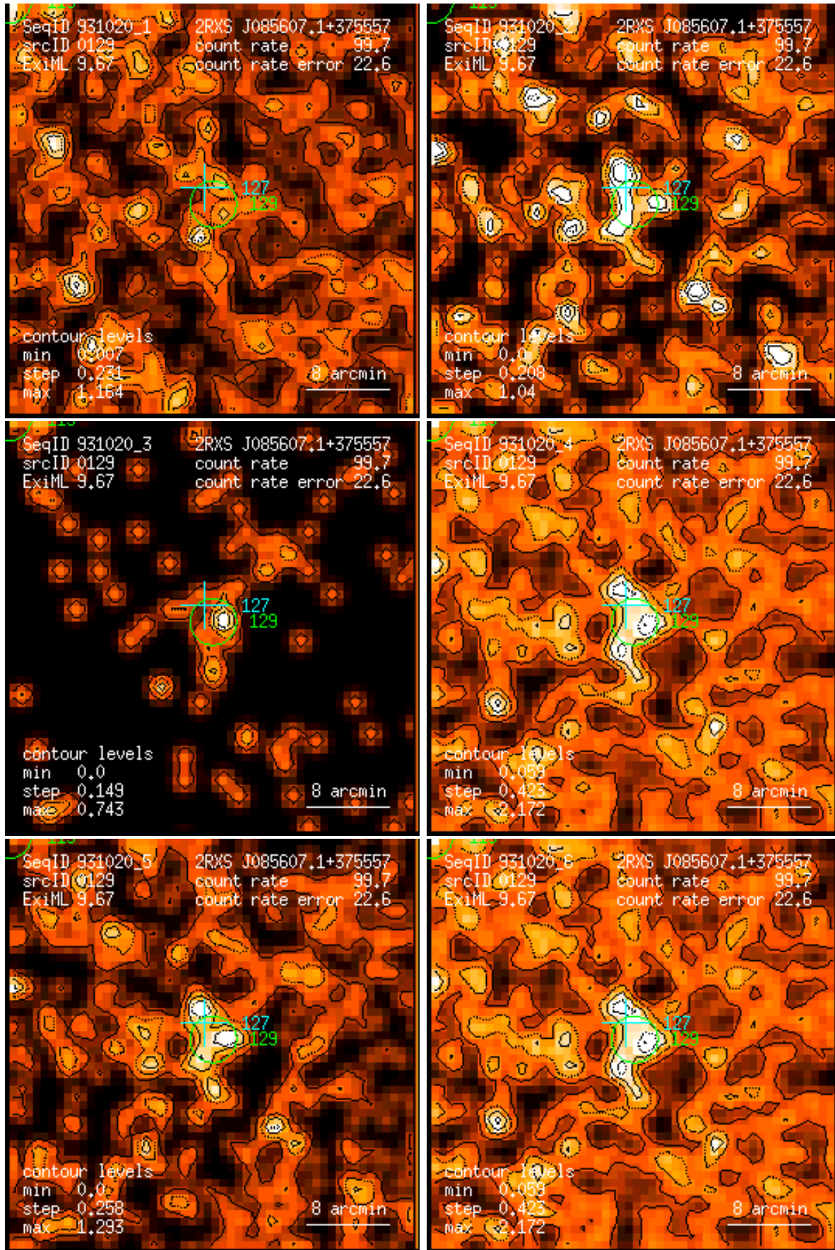
Figure 129: RASS 931020: detection 0129: band rate images, Gaussian filter: (1) PSPC channels 11 – 41, (2) 52 – 90, (3) 91 – 201, (4) 11 – 235, (5) 52 – 201, (6) 11 – 201. Broad band rates in counts/ks. Band rate contour levels in counts/ks/arcmin 2 .
