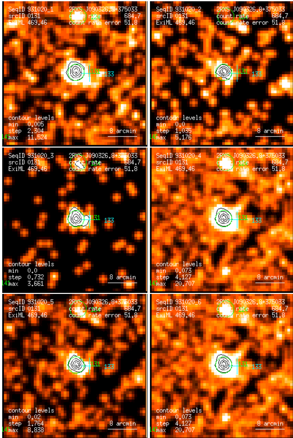
Figure 131: RASS 931020: detection 0131: band rate images, Gaussian filter: (1) PSPC channels 11 – 41, (2) 52 – 90, (3) 91 – 201, (4) 11 – 235, (5) 52 – 201, (6) 11 – 201. Broad band rates in counts/ks. Band rate contour levels in counts/ks/arcmin 2 .
