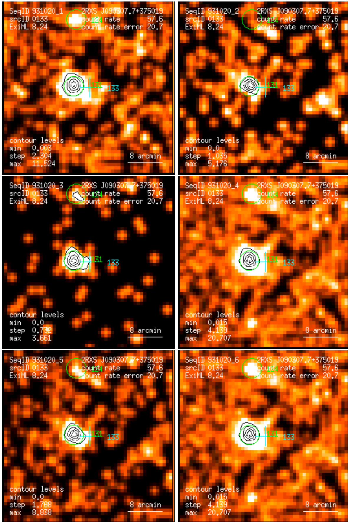
Figure 133: RASS 931020: detection 0133: band rate images, Gaussian filter: (1) PSPC channels 11 – 41, (2) 52 – 90, (3) 91 – 201, (4) 11 – 235, (5) 52 – 201, (6) 11 – 201. Broad band rates in counts/ks. Band rate contour levels in counts/ks/arcmin 2 .
