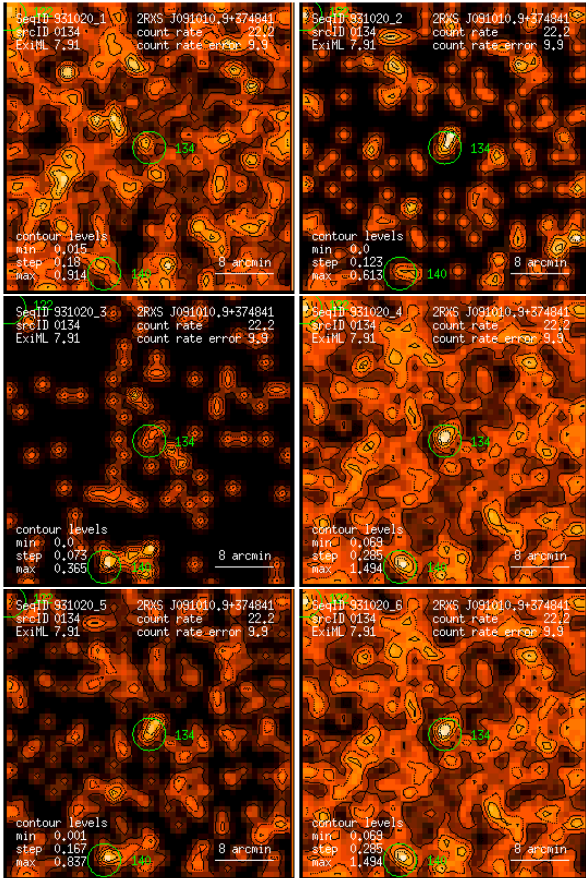
Figure 134: RASS 931020: detection 0134: band rate images, Gaussian filter: (1) PSPC channels 11 – 41, (2) 52 – 90, (3) 91 – 201, (4) 11 – 235, (5) 52 – 201, (6) 11 – 201. Broad band rates in counts/ks. Band rate contour levels in counts/ks/arcmin 2 .
