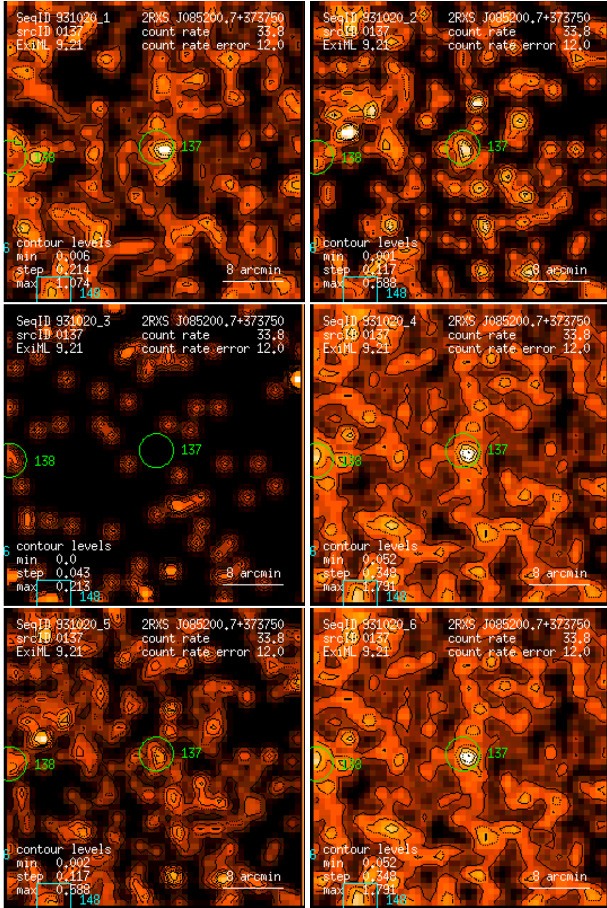
Figure 137: RASS 931020: detection 0137: band rate images, Gaussian filter: (1) PSPC channels 11 – 41, (2) 52 – 90, (3) 91 – 201, (4) 11 – 235, (5) 52 – 201, (6) 11 – 201. Broad band rates in counts/ks. Band rate contour levels in counts/ks/arcmin 2 .
