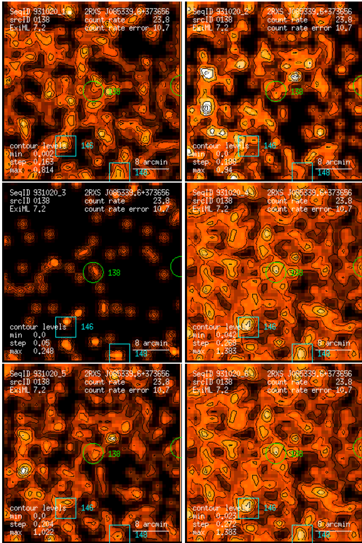
Figure 138: RASS 931020: detection 0138: band rate images, Gaussian filter: (1) PSPC channels 11 – 41, (2) 52 – 90, (3) 91 – 201, (4) 11 – 235, (5) 52 – 201, (6) 11 – 201. Broad band rates in counts/ks. Band rate contour levels in counts/ks/arcmin 2 .
