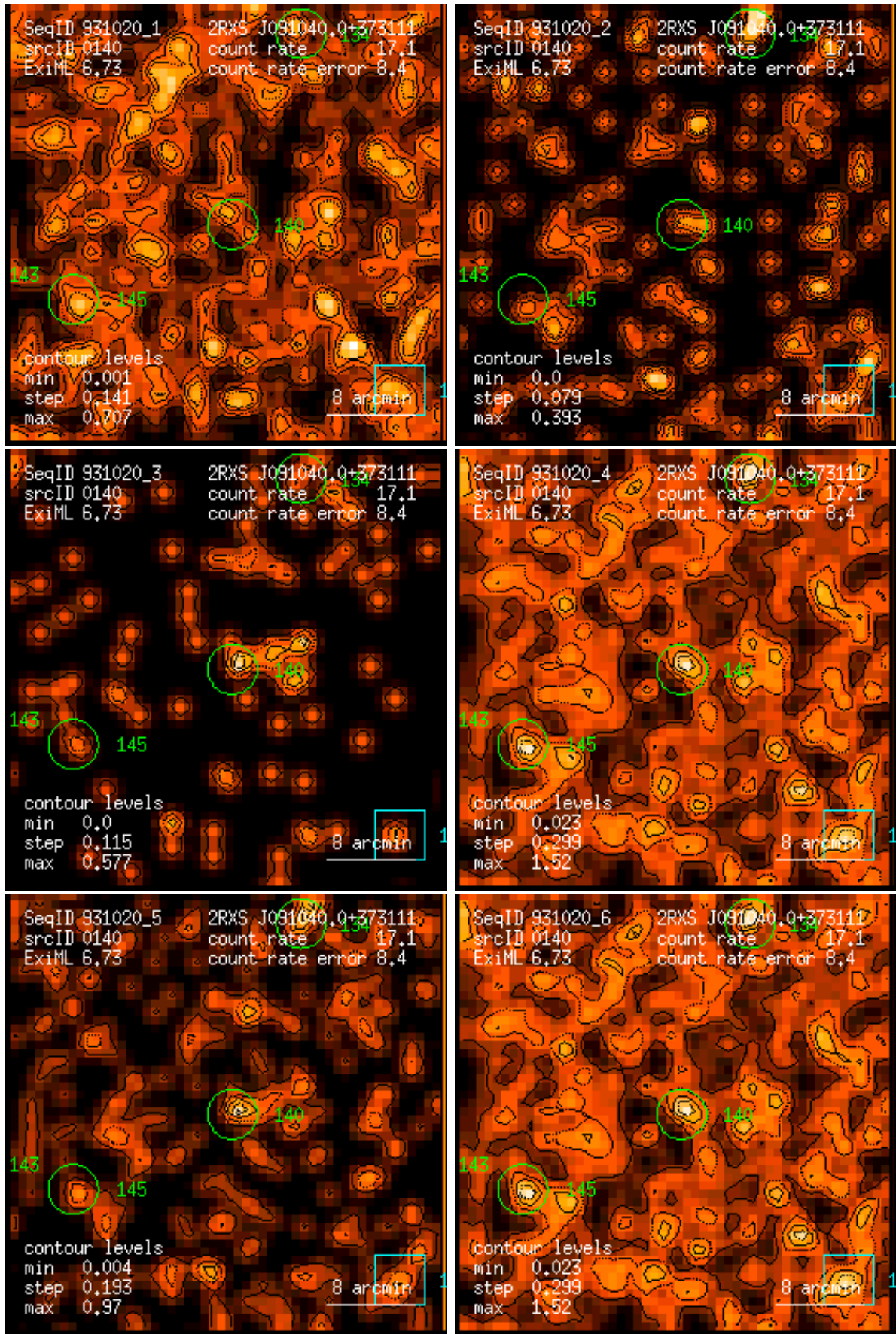
Figure 140: RASS 931020: detection 0140: band rate images, Gaussian filter: (1) PSPC channels 11 – 41, (2) 52 – 90, (3) 91 – 201, (4) 11 – 235, (5) 52 – 201, (6) 11 – 201. Broad band rates in counts/ks. Band rate contour levels in counts/ks/arcmin 2 .
