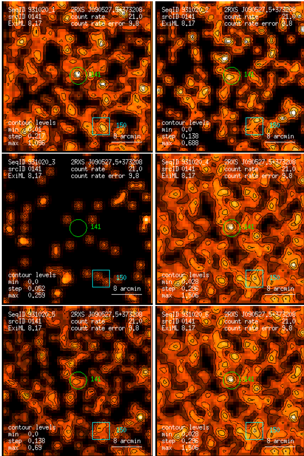
Figure 141: RASS 931020: detection 0141: band rate images, Gaussian filter: (1) PSPC channels 11 – 41, (2) 52 – 90, (3) 91 – 201, (4) 11 – 235, (5) 52 – 201, (6) 11 – 201. Broad band rates in counts/ks. Band rate contour levels in counts/ks/arcmin 2 .
