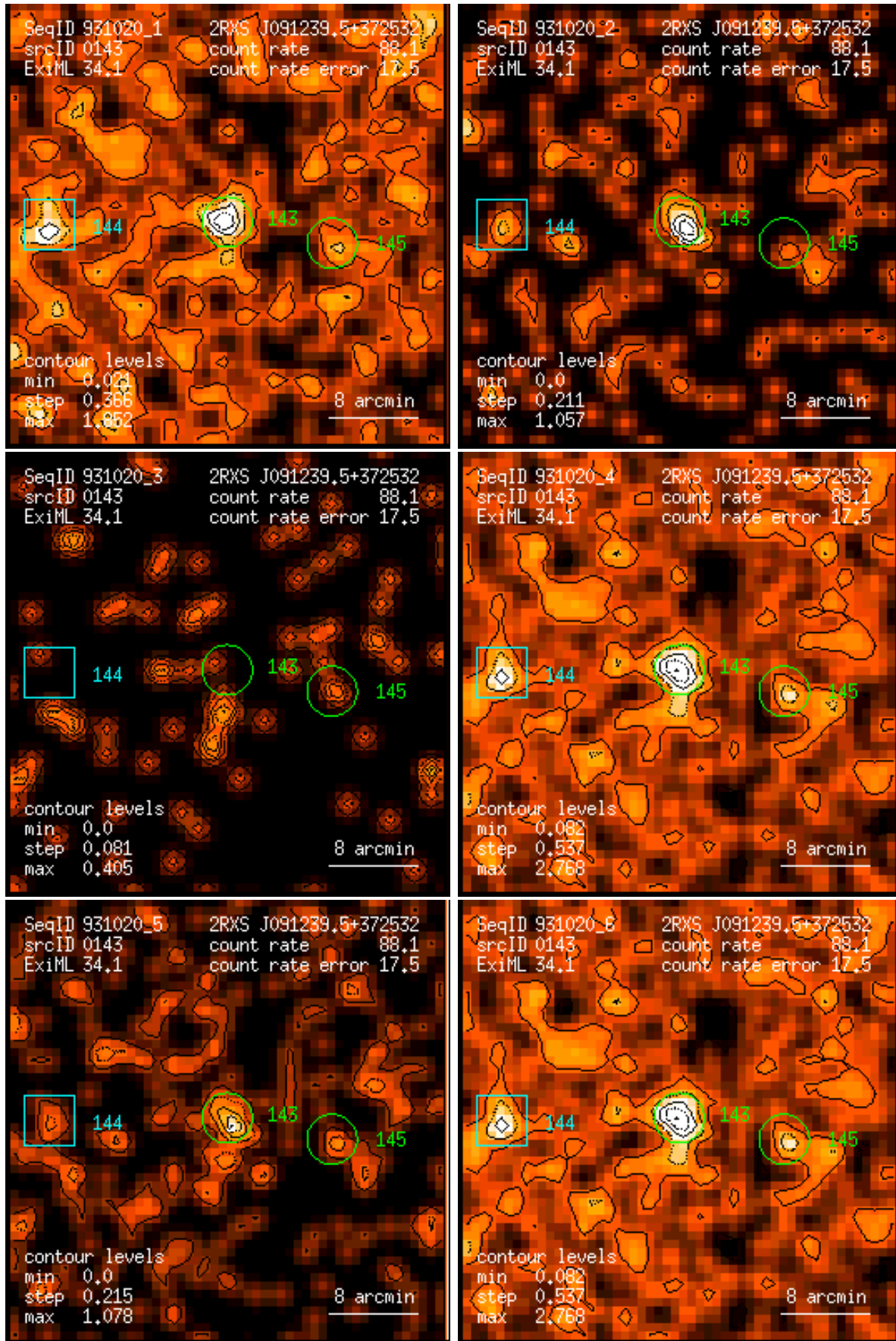
Figure 143: RASS 931020: detection 0143: band rate images, Gaussian filter: (1) PSPC channels 11 – 41, (2) 52 – 90, (3) 91 – 201, (4) 11 – 235, (5) 52 – 201, (6) 11 – 201. Broad band rates in counts/ks. Band rate contour levels in counts/ks/arcmin 2 .
