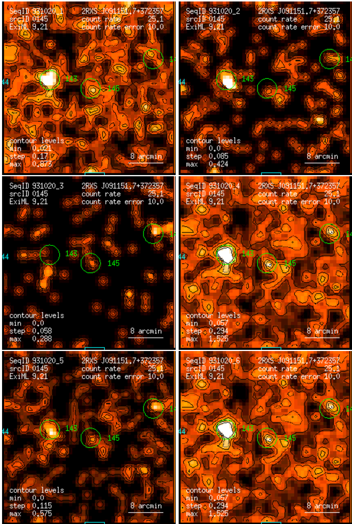
Figure 145: RASS 931020: detection 0145: band rate images, Gaussian filter: (1) PSPC channels 11 – 41, (2) 52 – 90, (3) 91 – 201, (4) 11 – 235, (5) 52 – 201, (6) 11 – 201. Broad band rates in counts/ks. Band rate contour levels in counts/ks/arcmin 2 .
