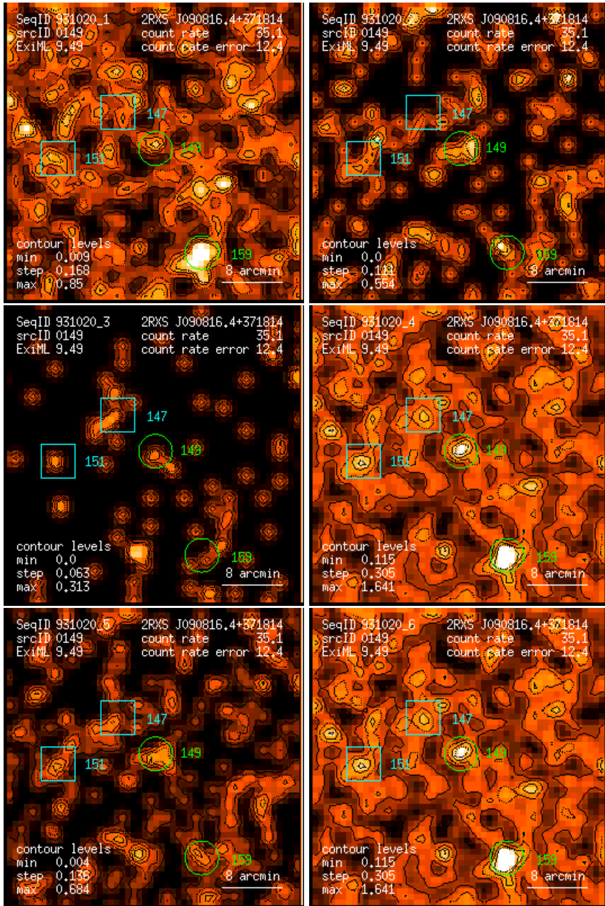
Figure 149: RASS 931020: detection 0149: band rate images, Gaussian filter: (1) PSPC channels 11 – 41, (2) 52 – 90, (3) 91 – 201, (4) 11 – 235, (5) 52 – 201, (6) 11 – 201. Broad band rates in counts/ks. Band rate contour levels in counts/ks/arcmin 2 .
