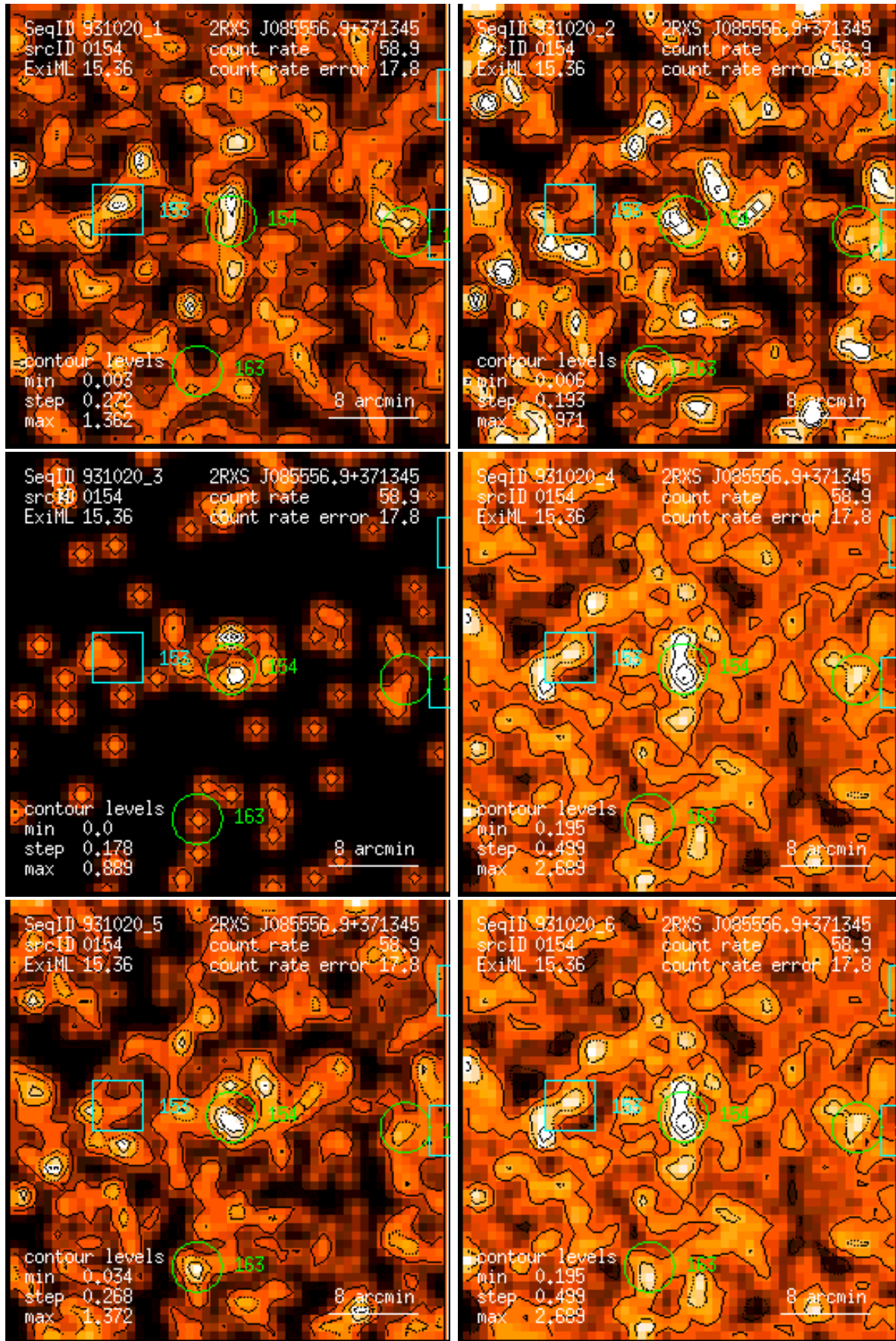
Figure 154: RASS 931020: detection 0154: band rate images, Gaussian filter: (1) PSPC channels 11 – 41, (2) 52 – 90, (3) 91 – 201, (4) 11 – 235, (5) 52 – 201, (6) 11 – 201. Broad band rates in counts/ks. Band rate contour levels in counts/ks/arcmin 2 .
