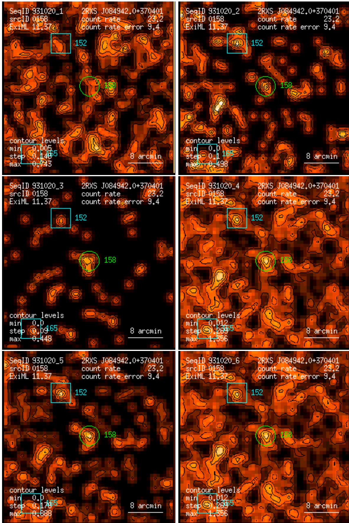
Figure 158: RASS 931020: detection 0158: band rate images, Gaussian filter: (1) PSPC channels 11 – 41, (2) 52 – 90, (3) 91 – 201, (4) 11 – 235, (5) 52 – 201, (6) 11 – 201. Broad band rates in counts/ks. Band rate contour levels in counts/ks/arcmin 2 .
