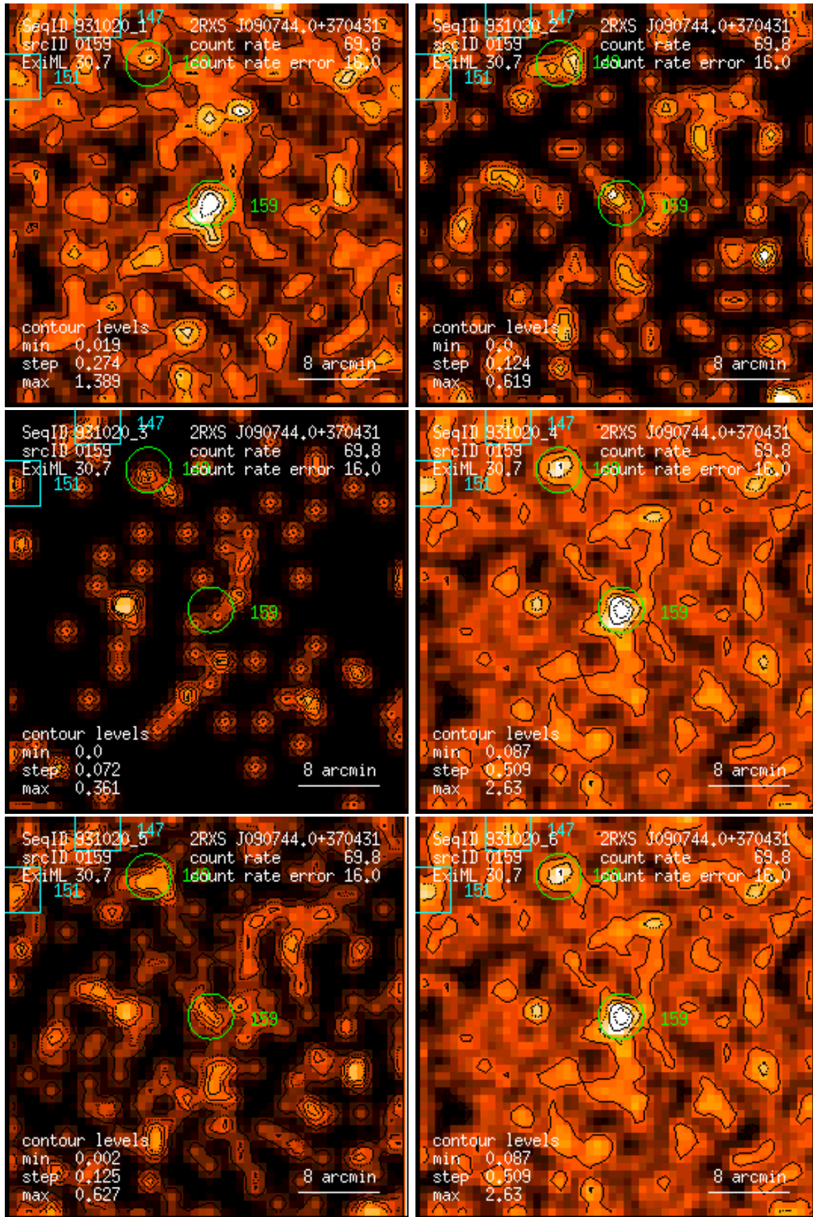
Figure 159: RASS 931020: detection 0159: band rate images, Gaussian filter: (1) PSPC channels 11 – 41, (2) 52 – 90, (3) 91 – 201, (4) 11 – 235, (5) 52 – 201, (6) 11 – 201. Broad band rates in counts/ks. Band rate contour levels in counts/ks/arcmin 2 .
