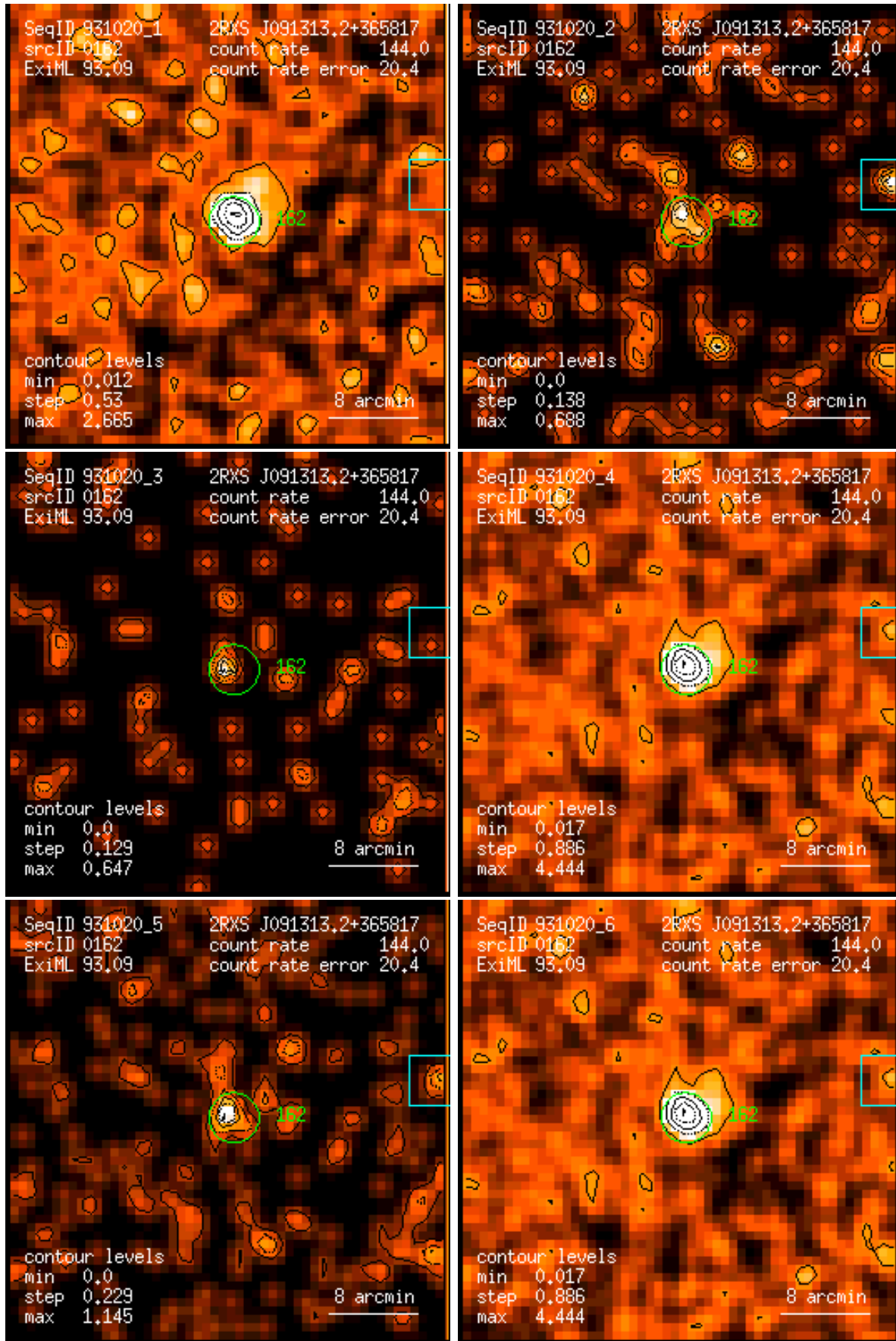
Figure 162: RASS 931020: detection 0162: band rate images, Gaussian filter: (1) PSPC channels 11 – 41, (2) 52 – 90, (3) 91 – 201, (4) 11 – 235, (5) 52 – 201, (6) 11 – 201. Broad band rates in counts/ks. Band rate contour levels in counts/ks/arcmin 2 .
