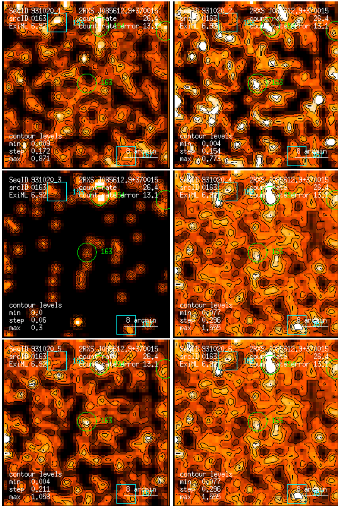
Figure 163: RASS 931020: detection 0163: band rate images, Gaussian filter: (1) PSPC channels 11 – 41, (2) 52 – 90, (3) 91 – 201, (4) 11 – 235, (5) 52 – 201, (6) 11 – 201. Broad band rates in counts/ks. Band rate contour levels in counts/ks/arcmin 2 .
