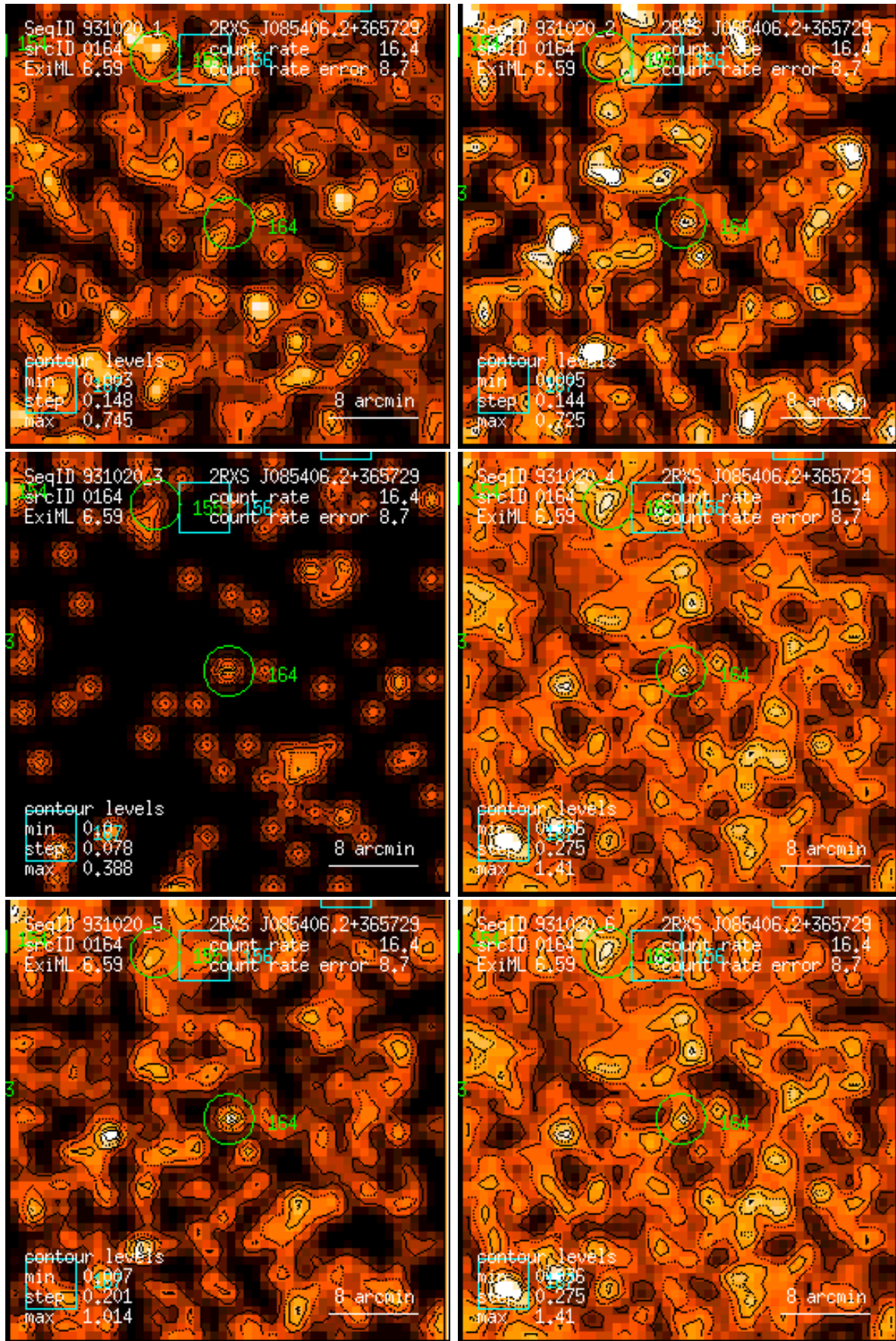
Figure 164: RASS 931020: detection 0164: band rate images, Gaussian filter: (1) PSPC channels 11 – 41, (2) 52 – 90, (3) 91 – 201, (4) 11 – 235, (5) 52 – 201, (6) 11 – 201. Broad band rates in counts/ks. Band rate contour levels in counts/ks/arcmin 2 .
