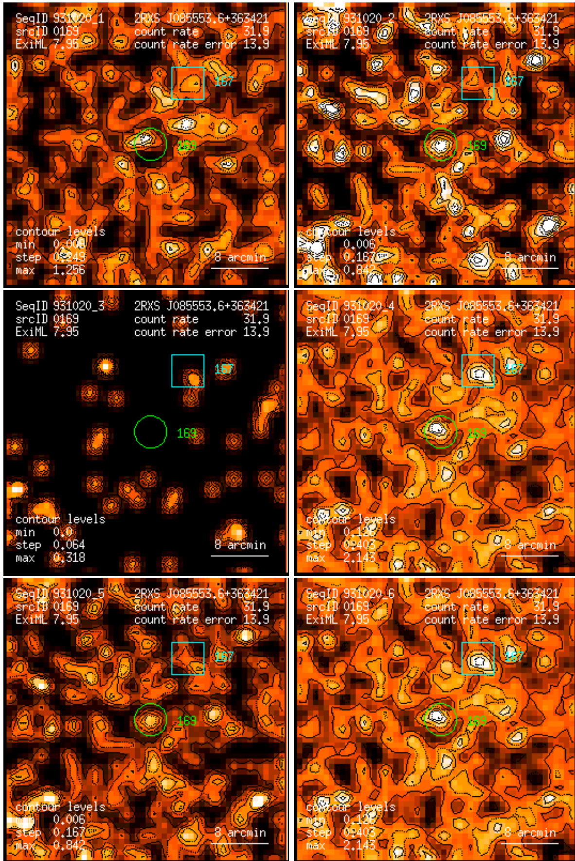
Figure 169: RASS 931020: detection 0169: band rate images, Gaussian filter: (1) PSPC channels 11 – 41, (2) 52 – 90, (3) 91 – 201, (4) 11 – 235, (5) 52 – 201, (6) 11 – 201. Broad band rates in counts/ks. Band rate contour levels in counts/ks/arcmin 2 .
