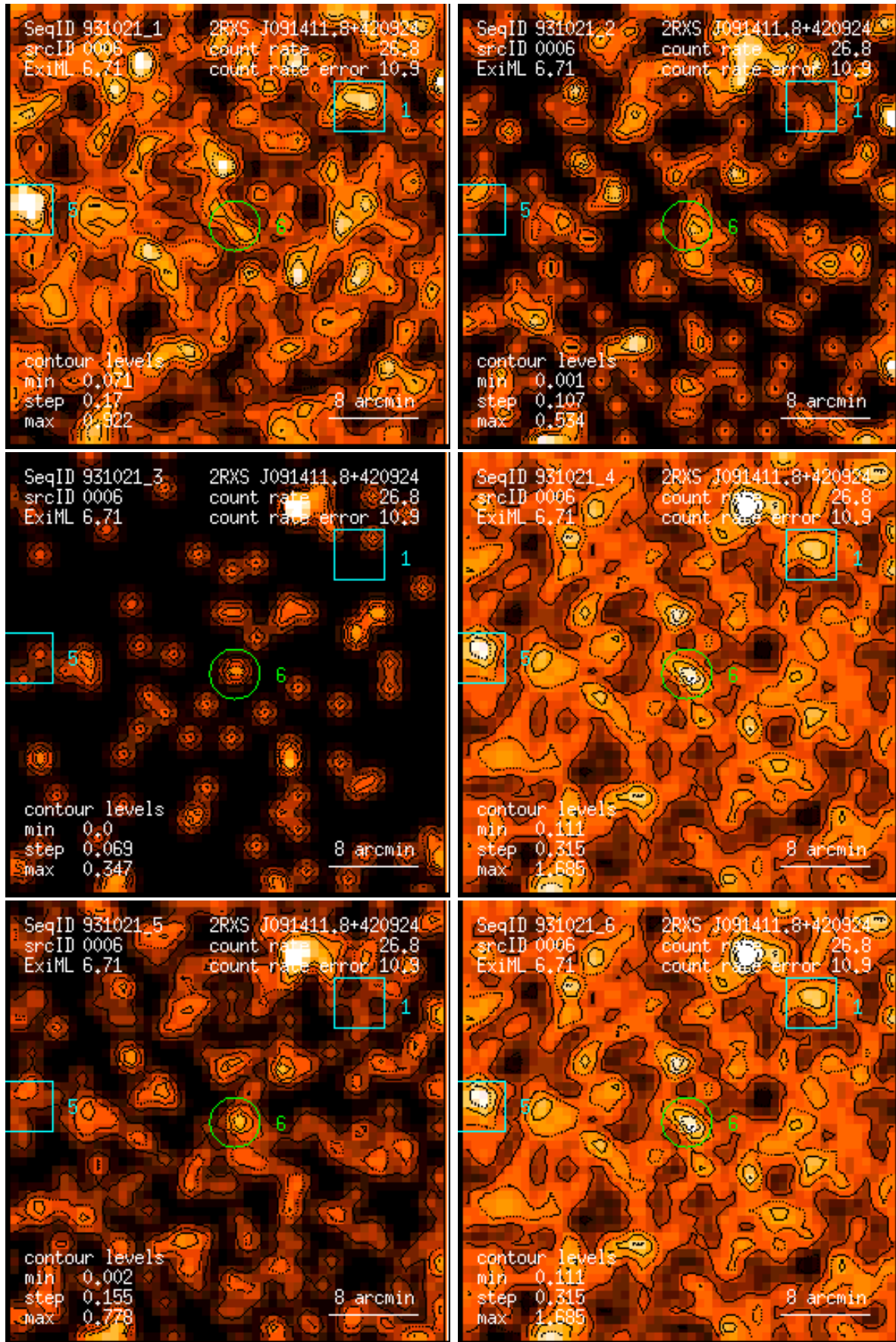
Figure 6: RASS 931021: detection 0006: band rate images, Gaussian filter: (1) PSPC channels 11 – 41, (2) 52 – 90, (3) 91 – 201, (4) 11 – 235, (5) 52 – 201, (6) 11 – 201. Broad band rates in counts/ks. Band rate contour levels in counts/ks/arcmin 2 .
