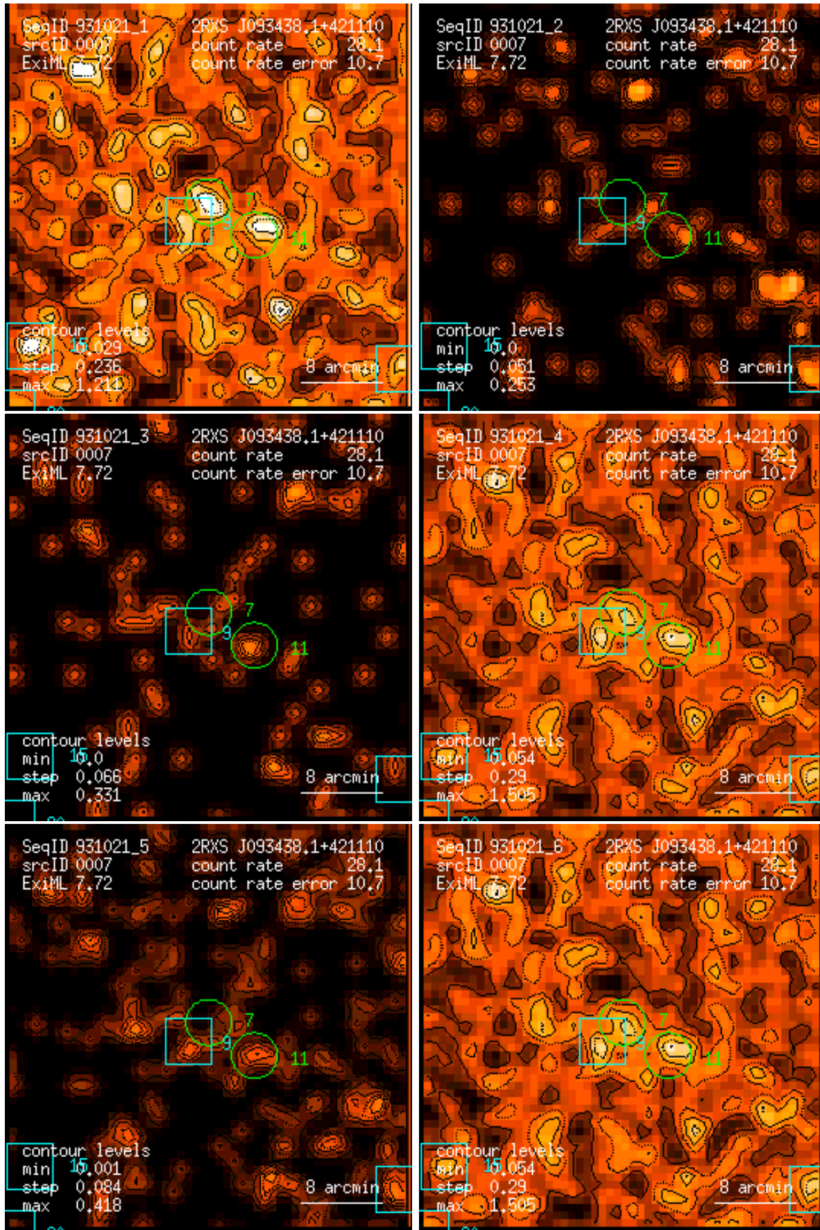
Figure 7: RASS 931021: detection 0007: band rate images, Gaussian filter: (1) PSPC channels 11 – 41, (2) 52 – 90, (3) 91 – 201, (4) 11 – 235, (5) 52 – 201, (6) 11 – 201. Broad band rates in counts/ks. Band rate contour levels in counts/ks/arcmin 2 .
