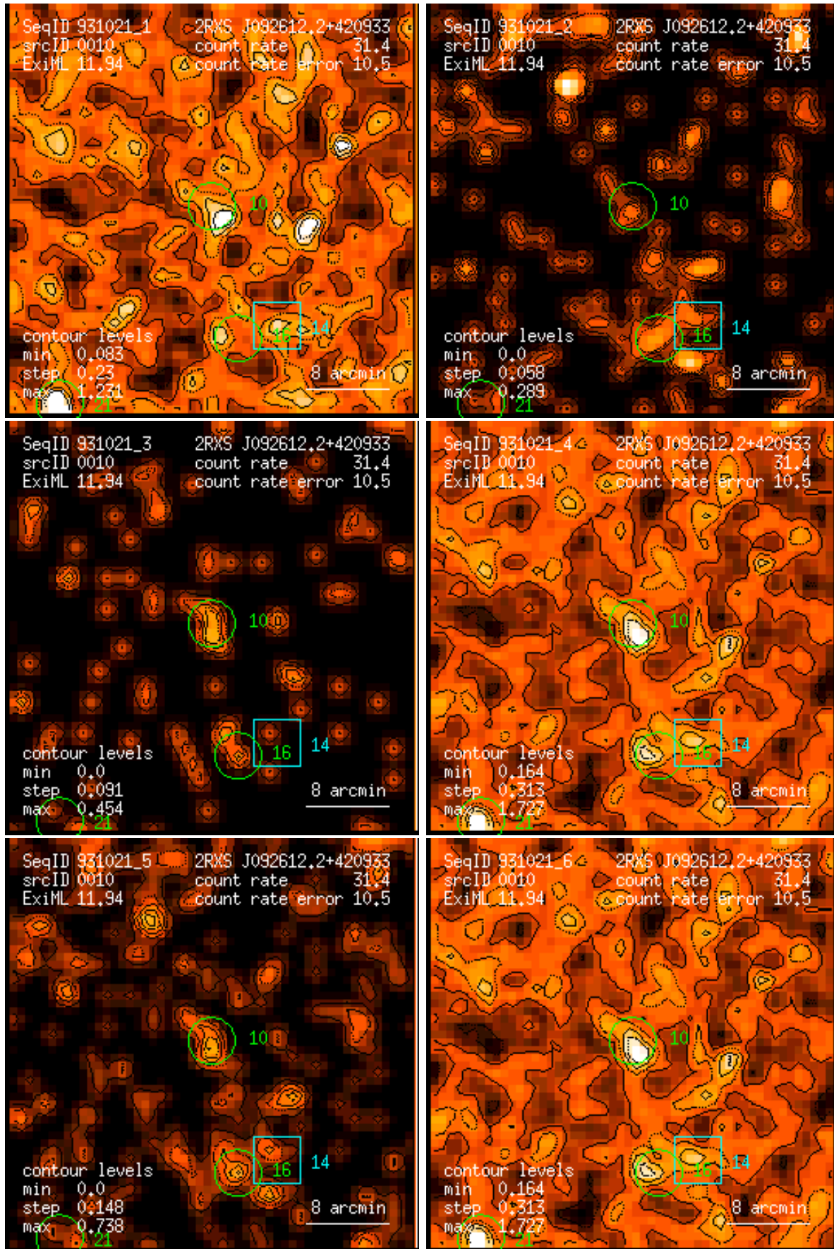
Figure 10: RASS 931021: detection 0010: band rate images, Gaussian filter: (1) PSPC channels 11 – 41, (2) 52 – 90, (3) 91 – 201, (4) 11 – 235, (5) 52 – 201, (6) 11 – 201. Broad band rates in counts/ks. Band rate contour levels in counts/ks/arcmin 2 .
