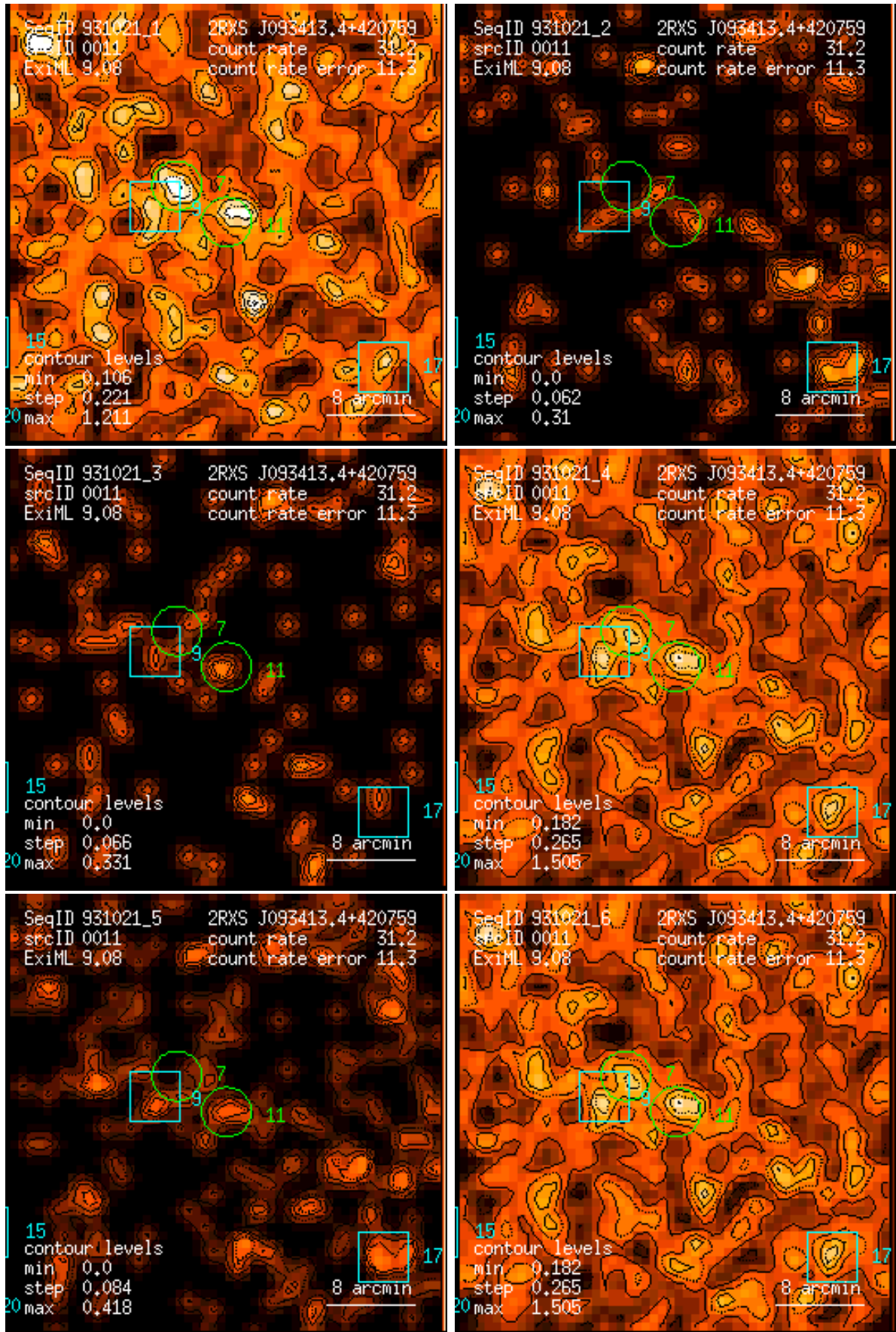
Figure 11: RASS 931021: detection 0011: band rate images, Gaussian filter: (1) PSPC channels 11 – 41, (2) 52 – 90, (3) 91 – 201, (4) 11 – 235, (5) 52 – 201, (6) 11 – 201. Broad band rates in counts/ks. Band rate contour levels in counts/ks/arcmin 2 .
