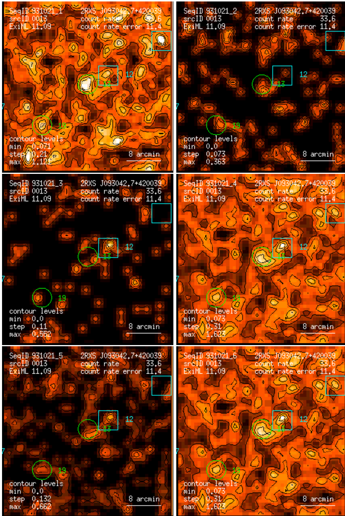
Figure 13: RASS 931021: detection 0013: band rate images, Gaussian filter: (1) PSPC channels 11 – 41, (2) 52 – 90, (3) 91 – 201, (4) 11 – 235, (5) 52 – 201, (6) 11 – 201. Broad band rates in counts/ks. Band rate contour levels in counts/ks/arcmin 2 .
